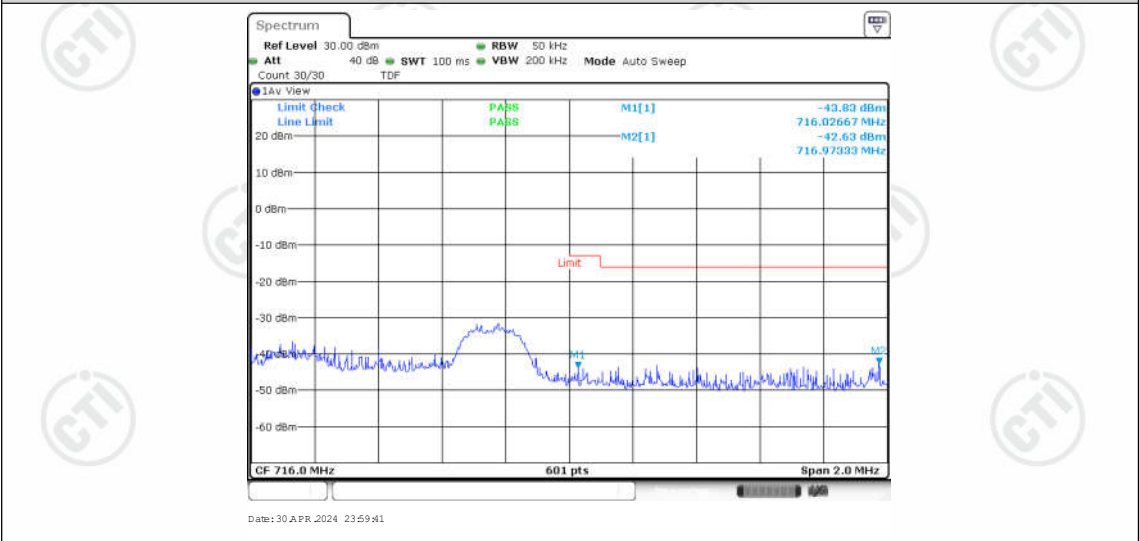
Band12-3MHz-16QAM-23165-1RB#14
