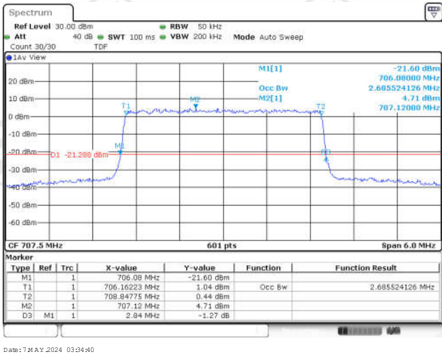
Band12-3MHz-16QAM-23165-15RB#0-2.686
