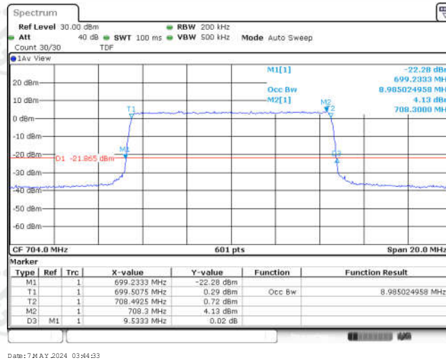
Band12-10MHz-QPSK-23095-50RB#0-8.985
