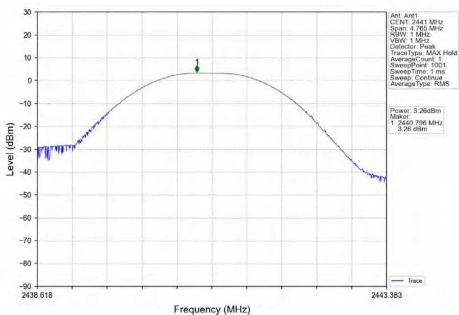
GFSK_DH5_MCH_2441MHz_Ant1_NTNV
