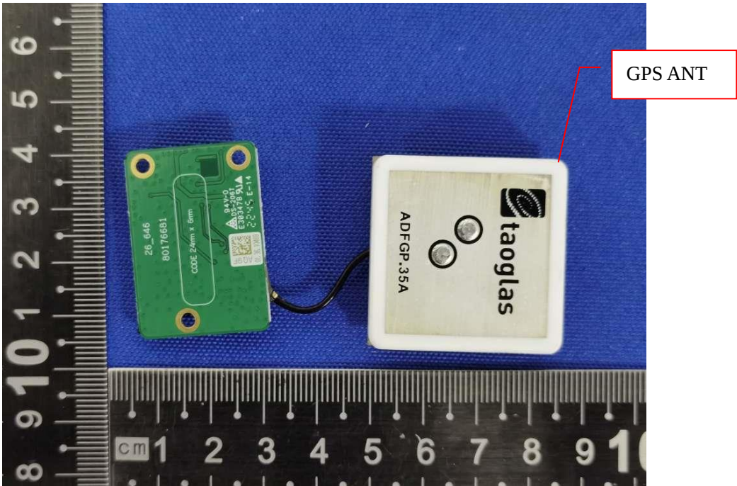
EUT Internal View 28
