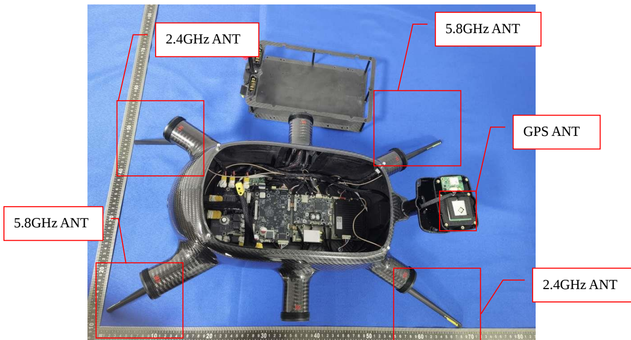
EUT Internal View 1
