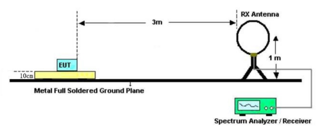
Figure 1. Below 30MHz
