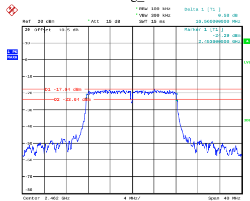
802.11g_2462MHz
