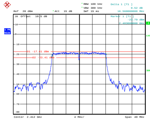
802.11g_2412MHz
