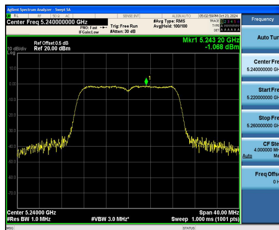
(802.11ac20) PSD plot on channel 48
