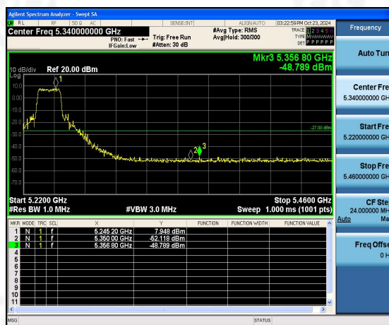
(802.11ac40) Band Edge, Right Side
