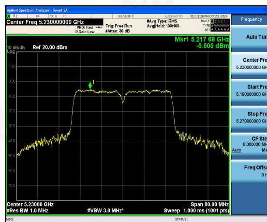
(802.11ac40) PSD plot on channel 46
