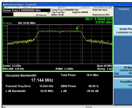
(802.11 a) 26dB Bandwidth plot on channel 40
