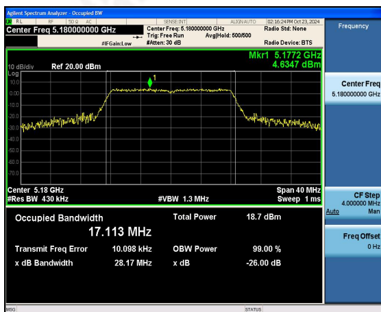
(802.11 a) 26dB Bandwidth plot on channel 36
