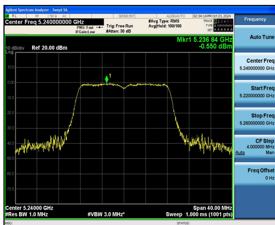
(802.11a) PSD plot on channel 48
