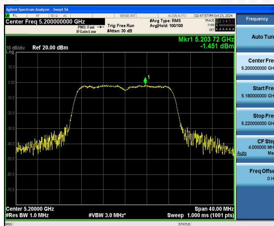
(802.11n20) PSD plot on channel 40
