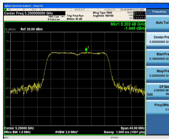
(802.11ac20) PSD plot on channel 40
