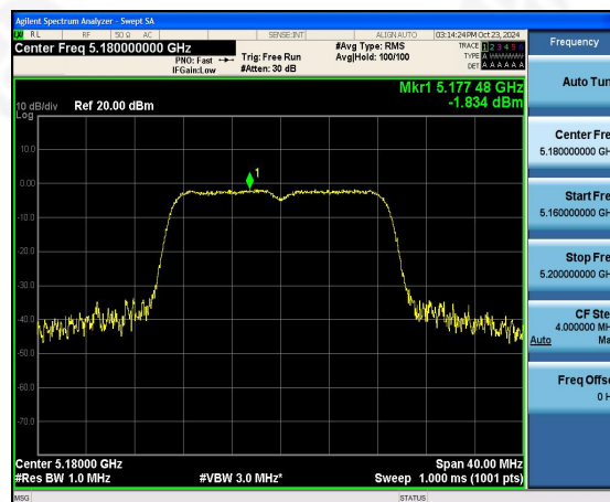
(802.11ac20) PSD plot on channel 36
