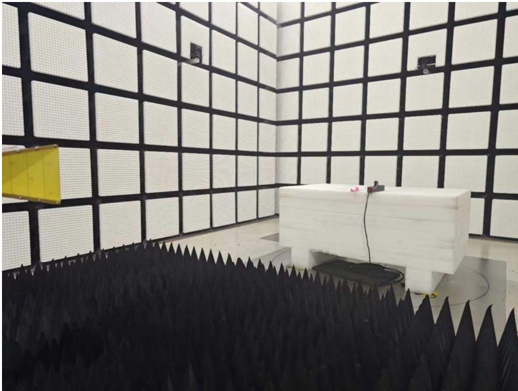
Radiated Emissions Above 1G Rear View-M1
