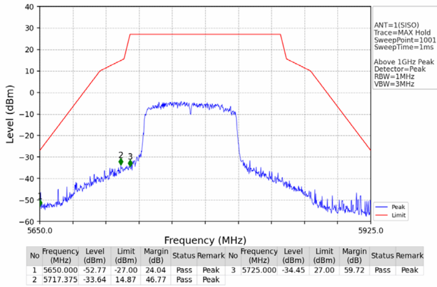
802.11ac(VHT80)_MCH_5775MHz_Ant1_NTNV
