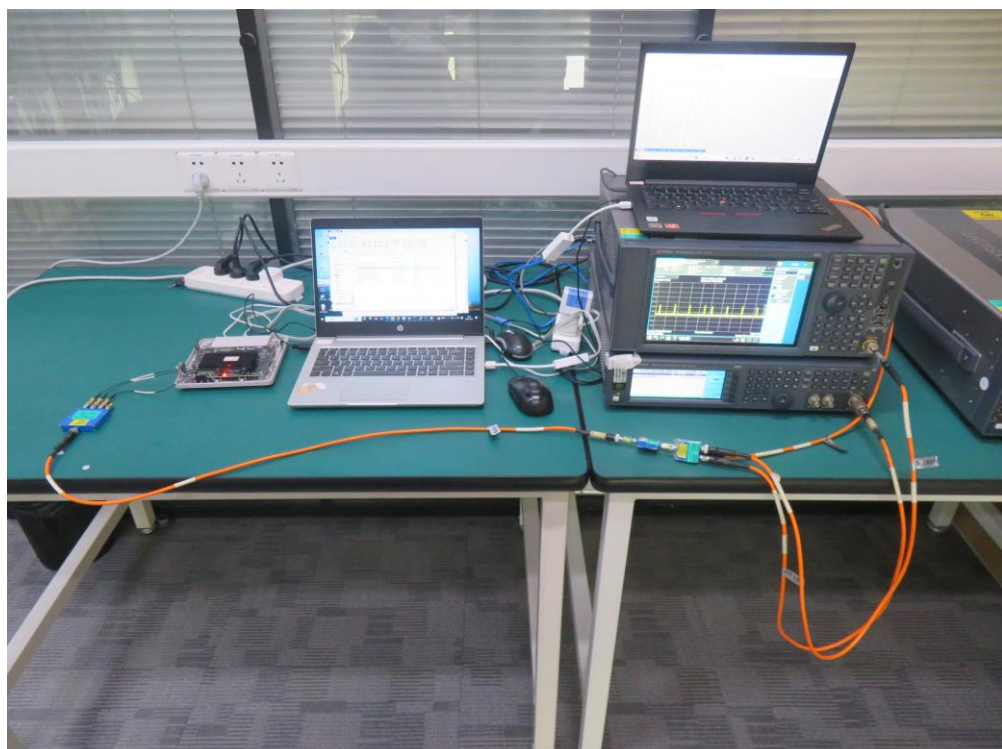
Description: DFS Test Setup (AP Mode)
