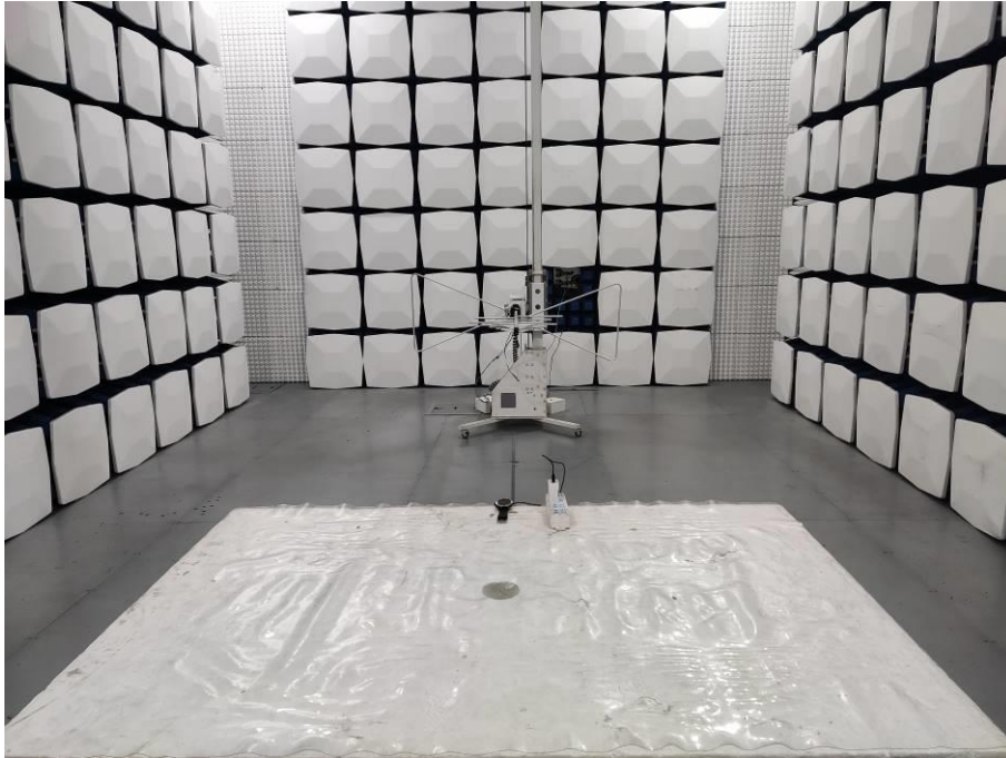
30MHz to 1GHz For BT test
