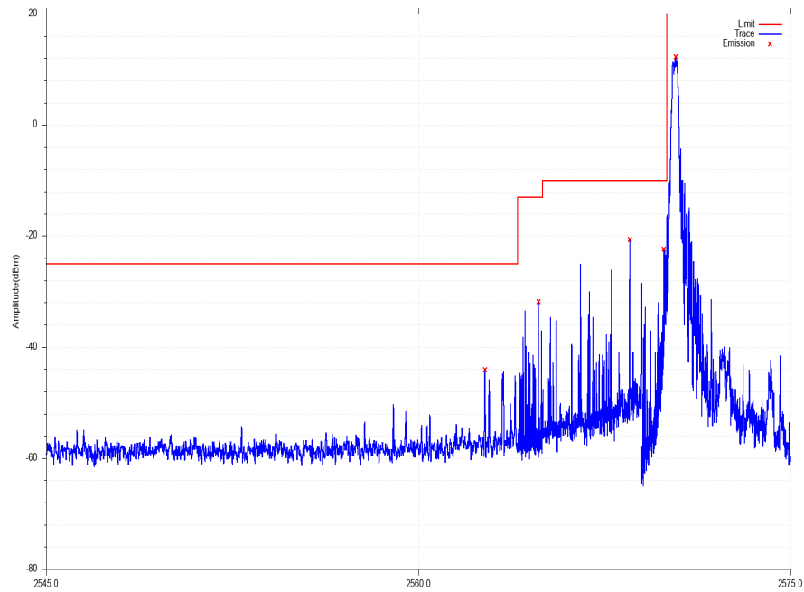
LOW_EDGE_Band_38_16QAM_5M_CH37775_1_0
