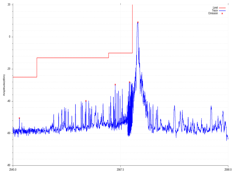
LOW_EDGE_Band_38_QPSK_20M_CH37850_1_0
