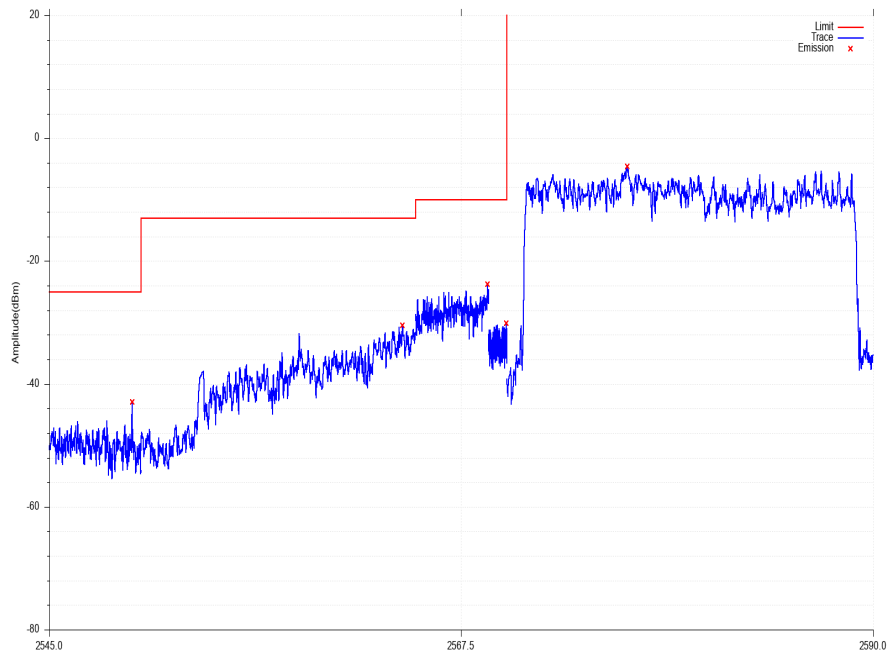
LOW_EDGE_Band_38_QPSK_20M_CH37850_100_0
