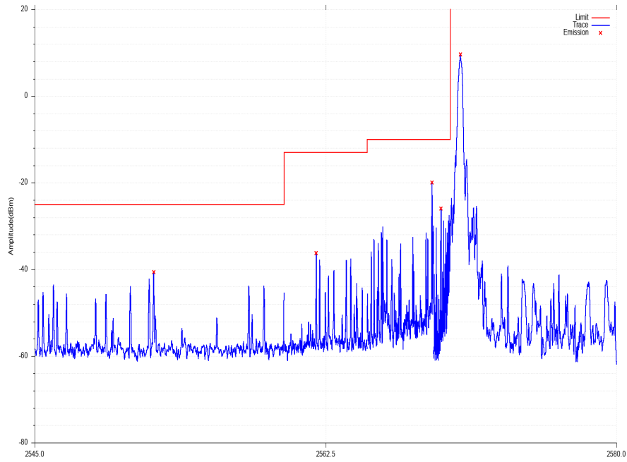
LOW_EDGE_Band_38_16QAM_10M_CH37800_1_0
