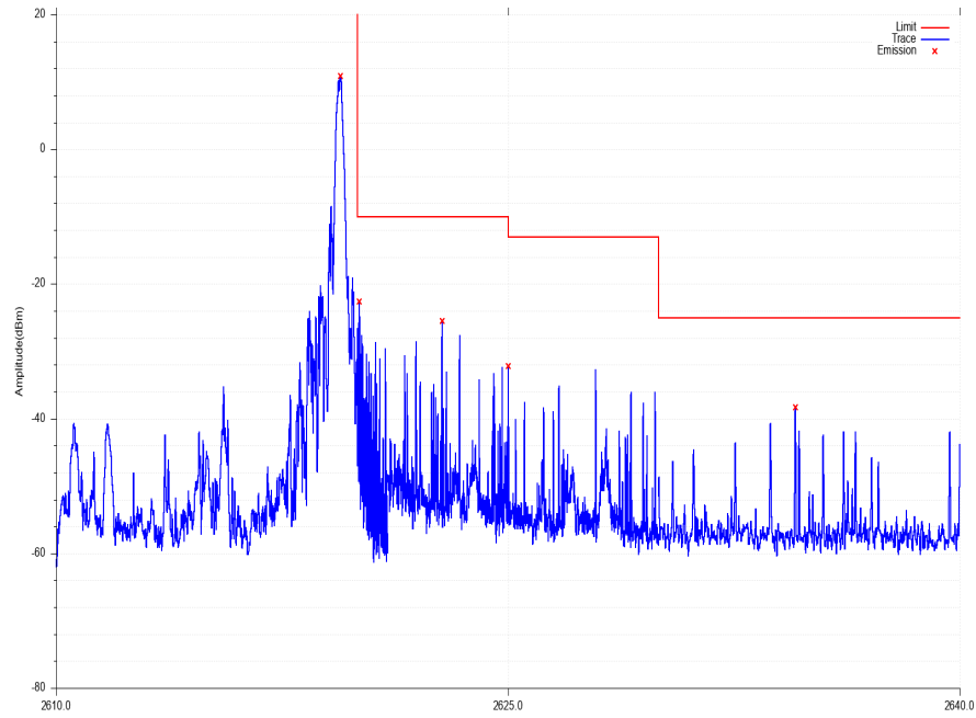
UP_EDGE_Band_38_16QAM_10M_CH38200_1_49
