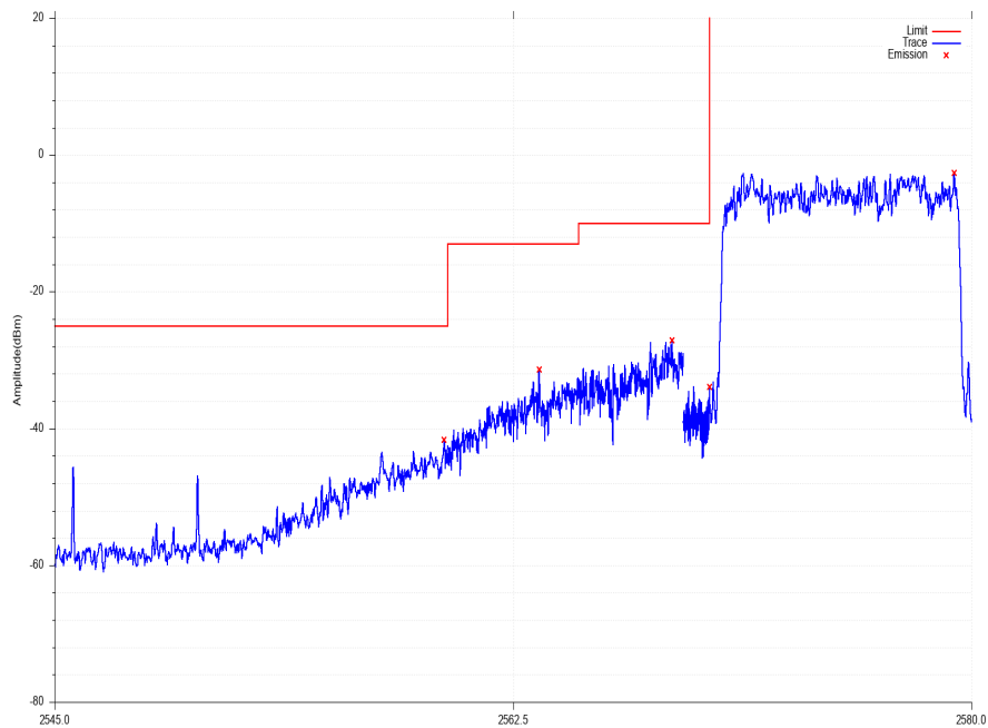
LOW_EDGE_Band_38_16QAM_10M_CH37800_50_0
