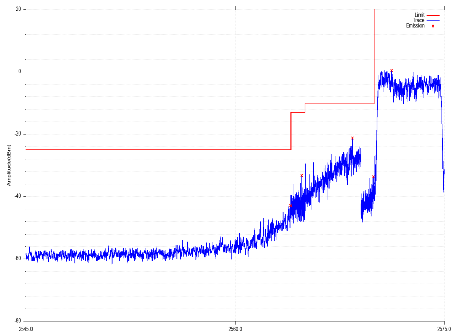
LOW_EDGE_Band_38_16QAM_5M_CH37775_25_0
