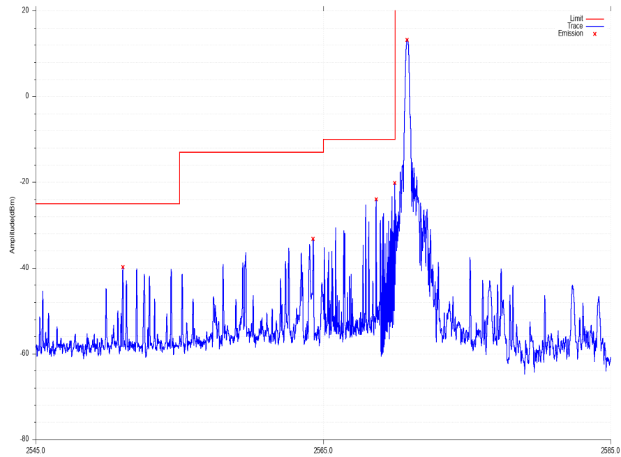
LOW_EDGE_Band_38_16QAM_15M_CH37825_1_0
