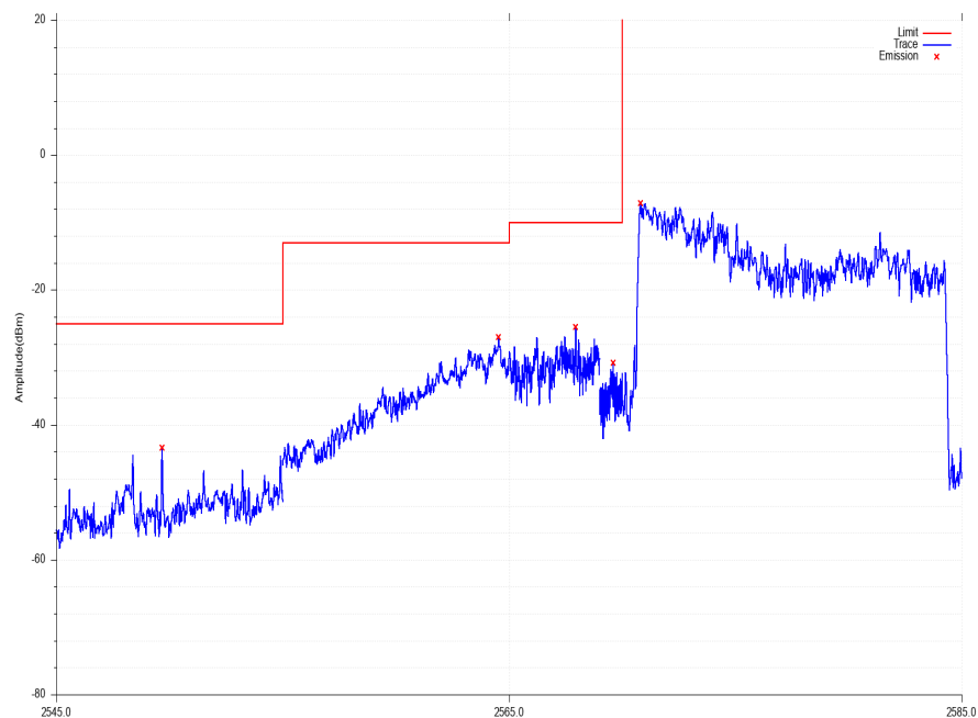
LOW_EDGE_Band_38_16QAM_15M_CH37825_75_0
