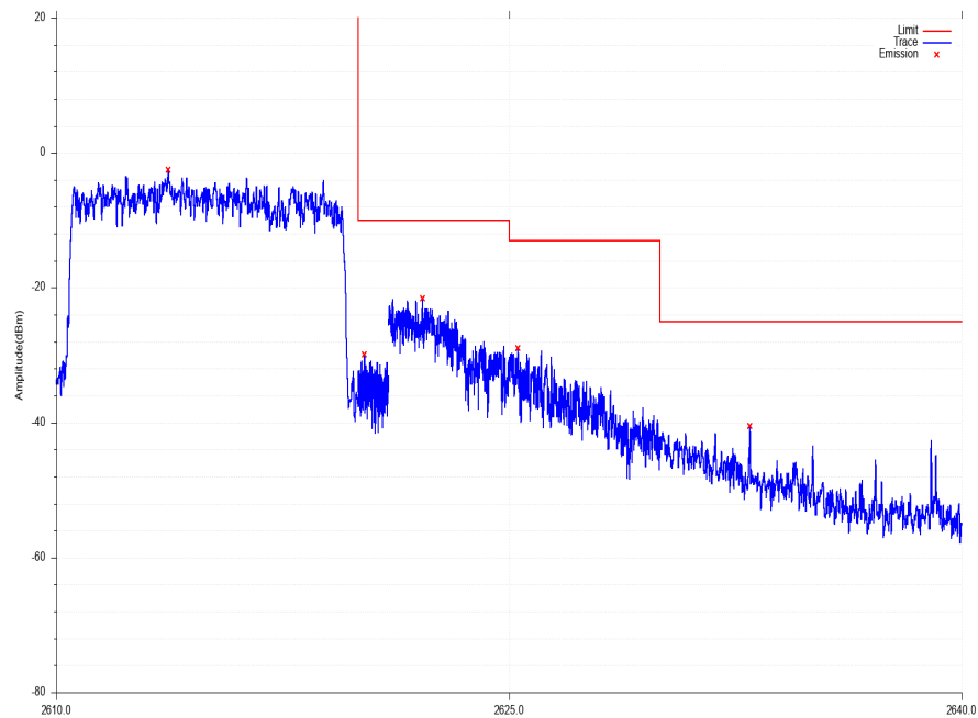
UP_EDGE_Band_38_16QAM_10M_CH38200_50_0
