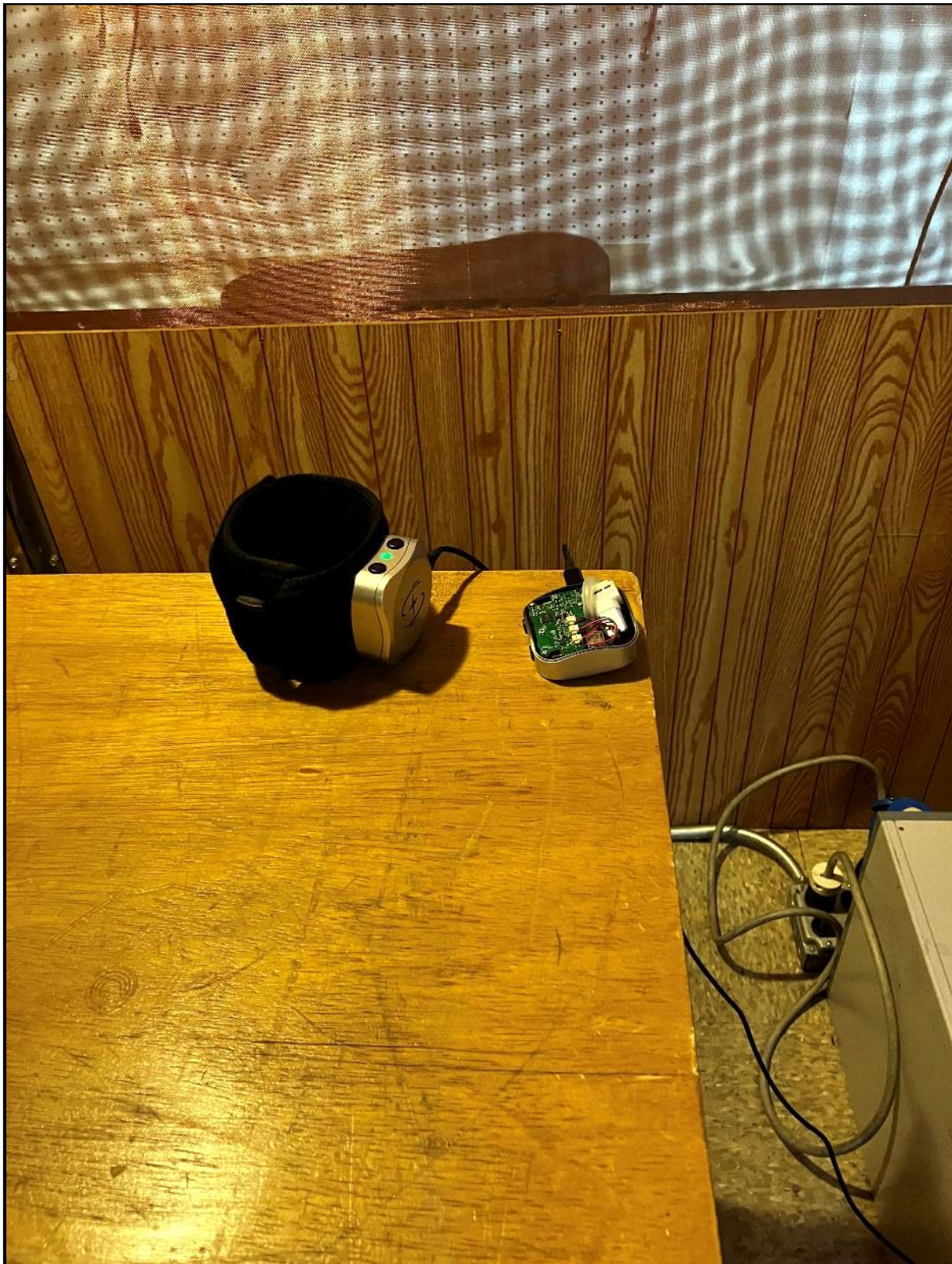
Photograph 5: AC Conducted Emissions - Front View
