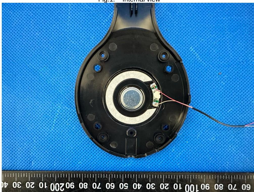
Fig.2. Speaker view
