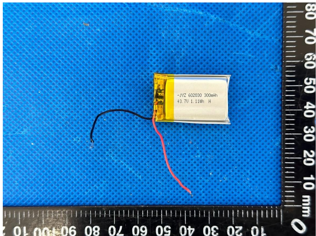
Fig.5. Battery view
