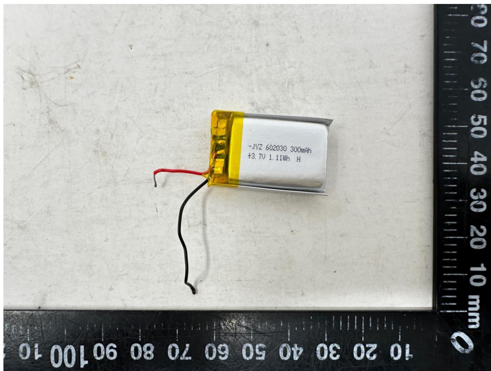
Fig.3. Battery view
