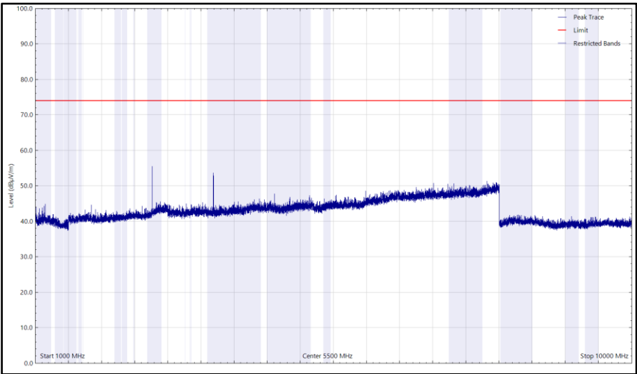
Figure 6 - ISM_UWB, 921.5_6489.6 MHz, 1 GHz to 10 GHz, Vertical (Peak)
