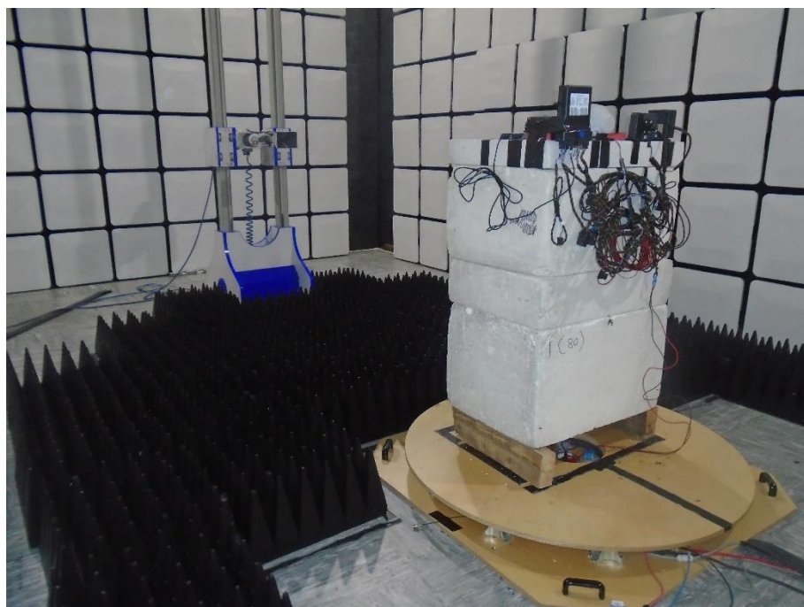
Figure 3 - Test Setup - 1 GHz to 10 GHz
