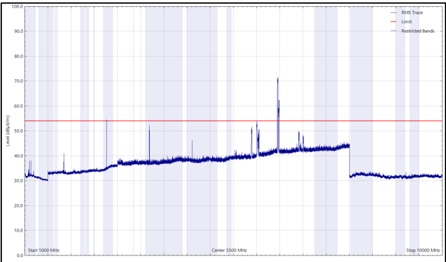
Figure 7 - ISM_UWB, 921.5_6489.6 MHz, 1 GHz to 10 GHz, Vertical (rms)
