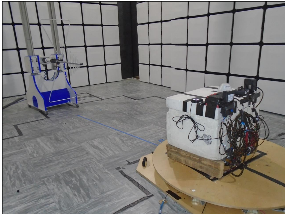
Figure 2 - Test Setup - 30 MHz to 1 GHz
