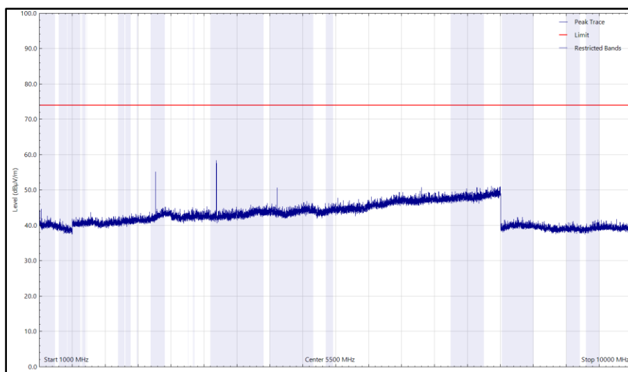
Figure 3 - ISM_UWB, 921.5_6489.6 MHz, 1 GHz to 10 GHz, Horizontal (Peak)
