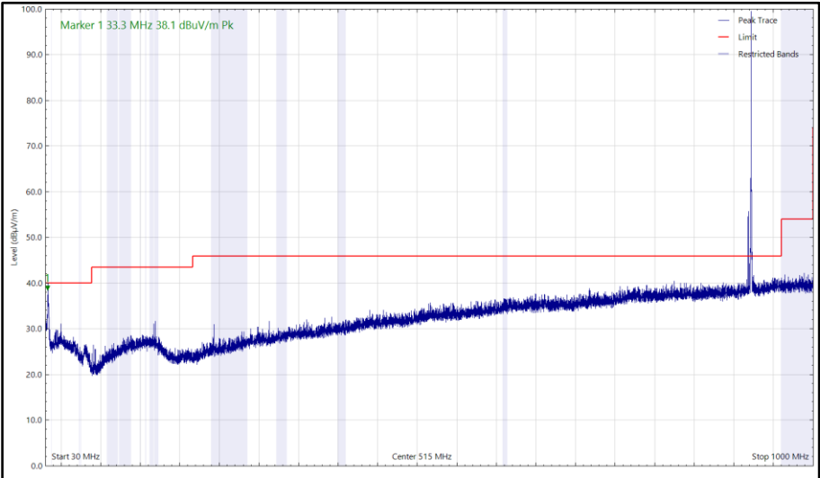
Figure 5 - ISM_UWB, 921.5_6489.6 MHz, 30 MHz to 1 GHz, Vertical (Peak)
