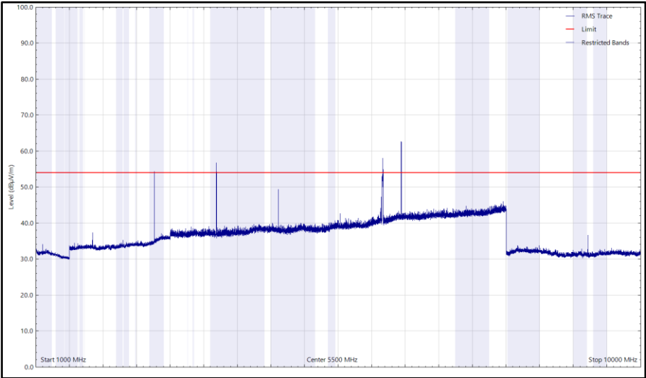
Figure 4 - ISM_UWB, 921.5_6489.6 MHz, 1 GHz to 10 GHz, Horizontal (rms)
