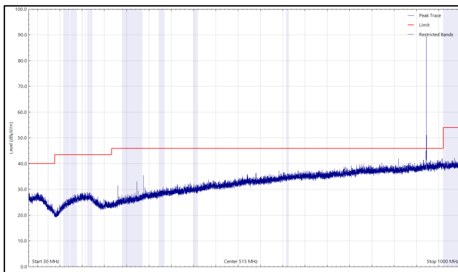
Figure 2 - ISM_UWB, 921.5_6489.6 MHz, 30 MHz to 1 GHz, Horizontal (Peak)
