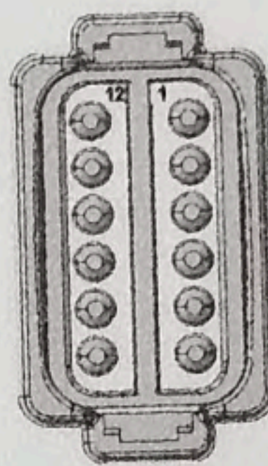
CAN SYSTEM
