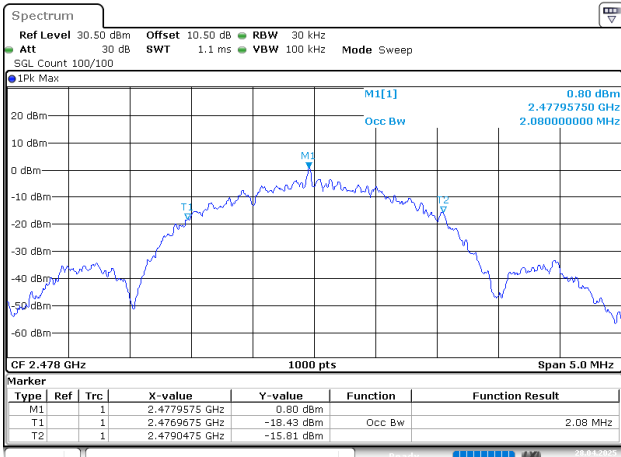
BLE_2M_High_Channel
