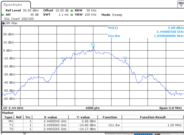
BLE_1M_Middle_Channel
