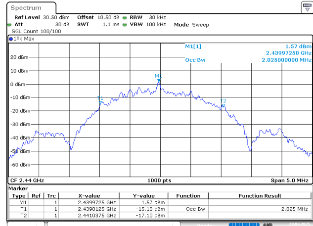
BLE_2M_Middle_Channel
