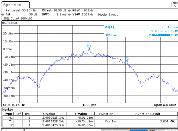
BLE_2M_Low_Channel
