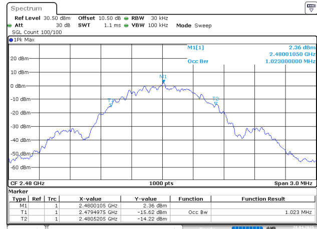
BLE_1M_High_Channel
