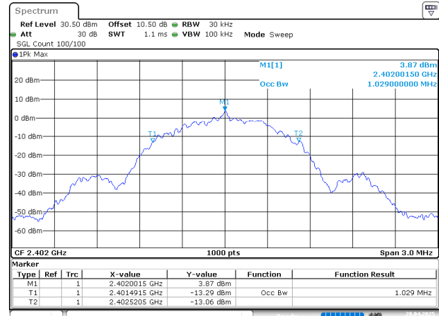
BLE_1M_Low_Channel
