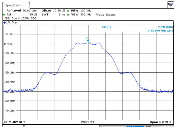
BLE_1M_Low_Channel
