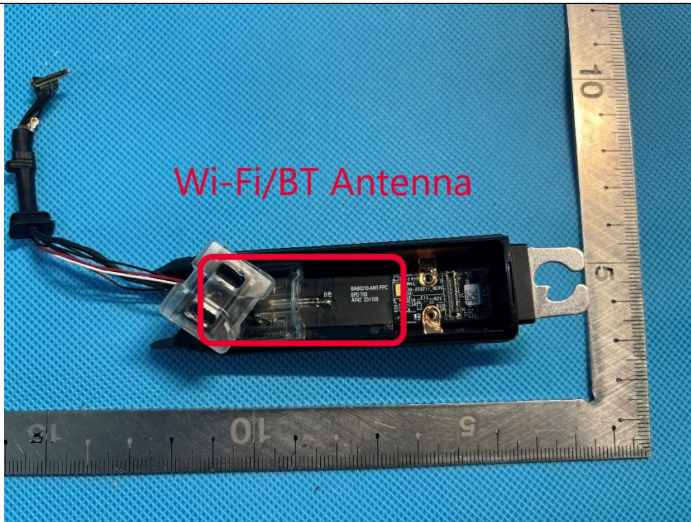
EUT Photo(14) Antenna WiFi 2
