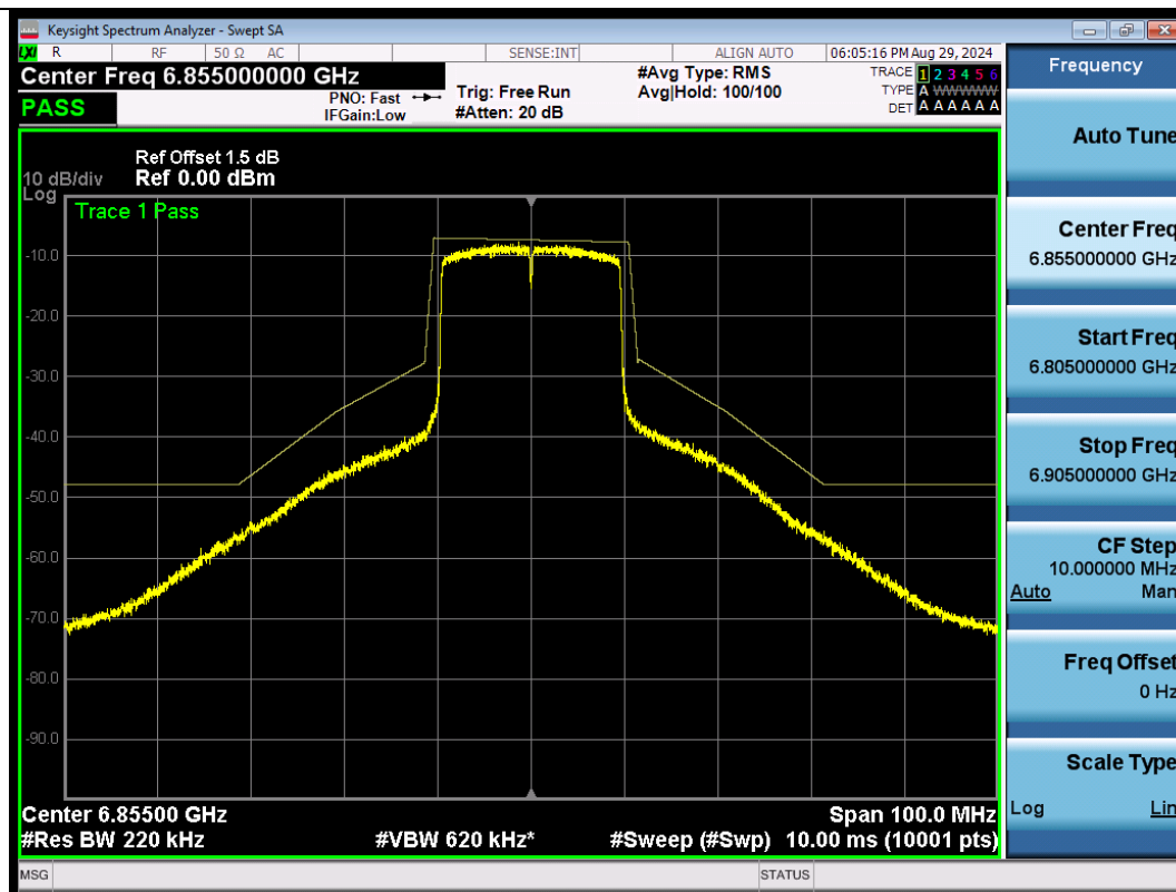
NTNV-11AX20SISO-Ant1-6855-PASS
