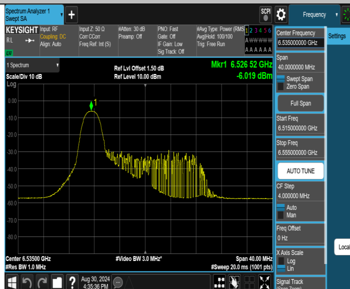
11AX20SISO_Ant1_6535_52Tone_RU37
