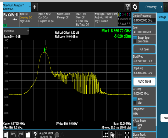
11AX20SISO_Ant1_6875_52Tone_RU37
