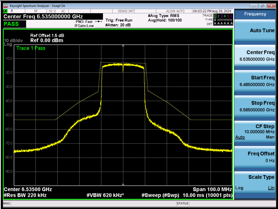
NTNV-11AX20SISO-Ant1-6535-PASS
