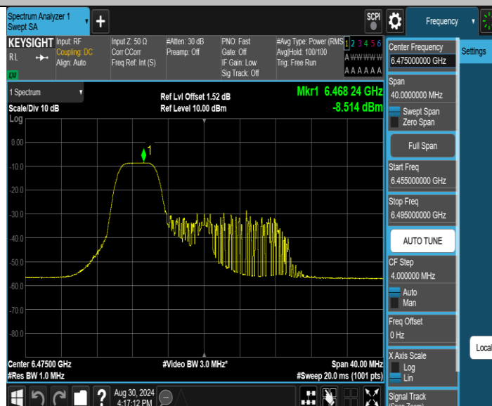
11AX20SISO_Ant1_6475_106Tone_RU53
