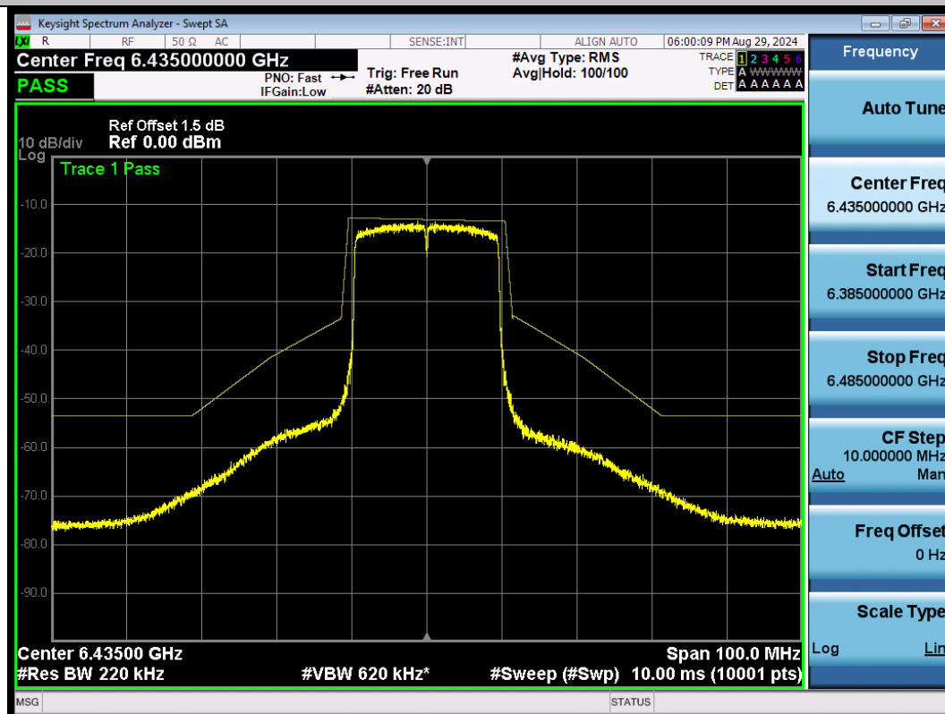
NTNV-11AX20SISO-Ant1-6435-PASS
