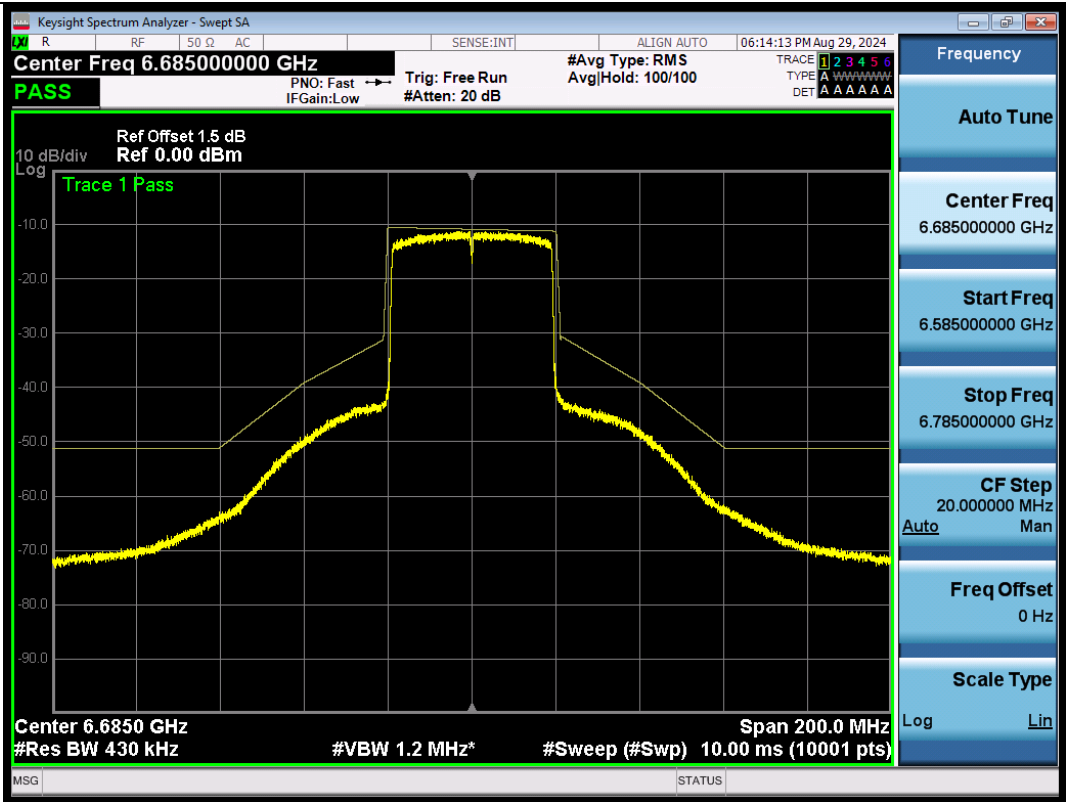
NTNV-11AX40SISO-Ant1-6685-PASS
