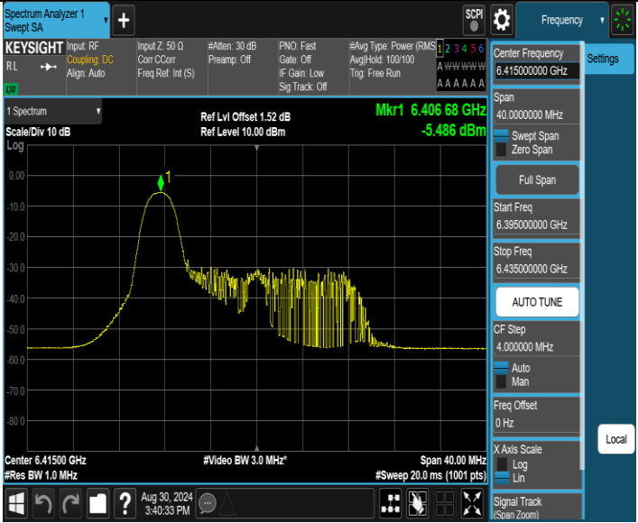
11AX20SISO_Ant1_6415_52Tone_RU37
