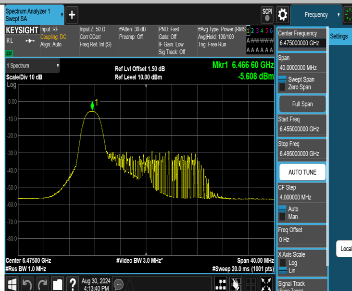
11AX20SISO_Ant1_6475_52Tone_RU37
