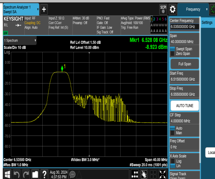
11AX20SISO_Ant1_6535_106Tone_RU53
