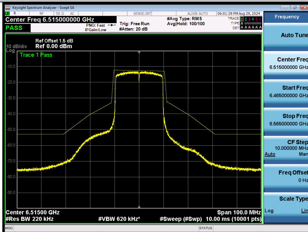
NTNV-11AX20SISO-Ant1-6515-PASS
