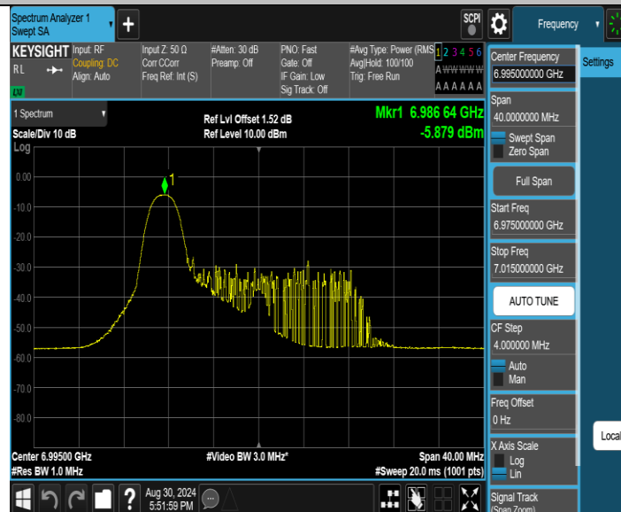
11AX20SISO_Ant1_6995_52Tone_RU37
