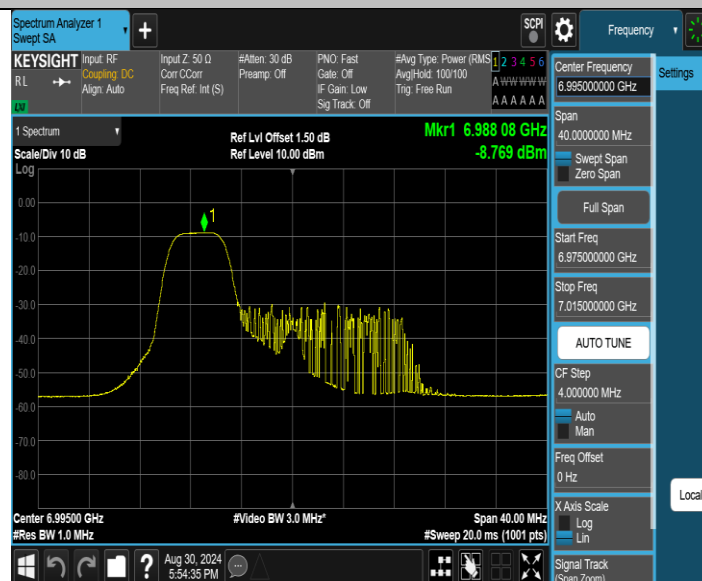
11AX20SISO_Ant1_6995_106Tone_RU53
