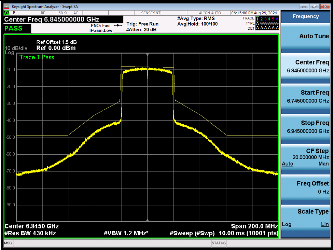
NTNV-11AX40SISO-Ant1-6845-PASS
