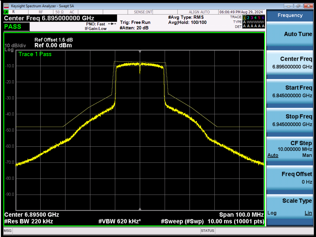
NTNV-11AX20SISO-Ant1-6895-PASS
