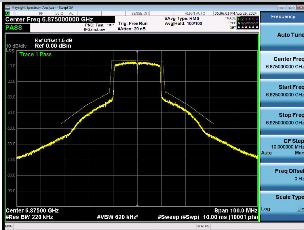
NTNV-11AX20SISO-Ant1-6875-PASS
