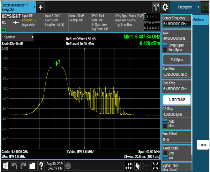
11AX20SISO_Ant1_6415_106Tone_RU53
