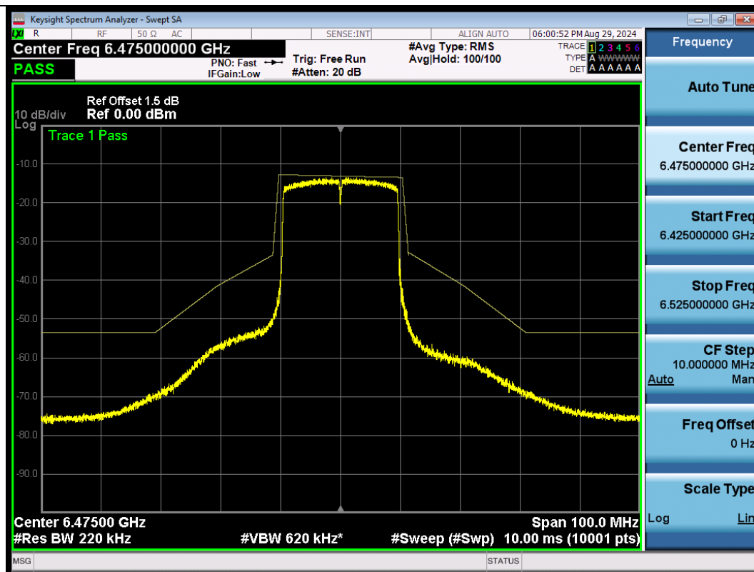
NTNV-11AX20SISO-Ant1-6475-PASS
