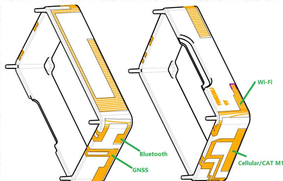
Figure 12.2-3 Antenna Locations
