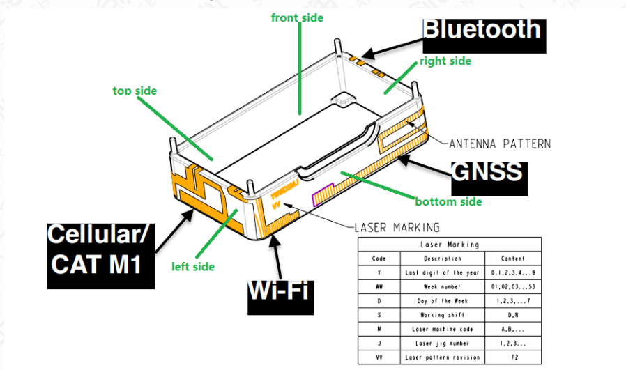
Figure 12.2-2 Antenna Locations
