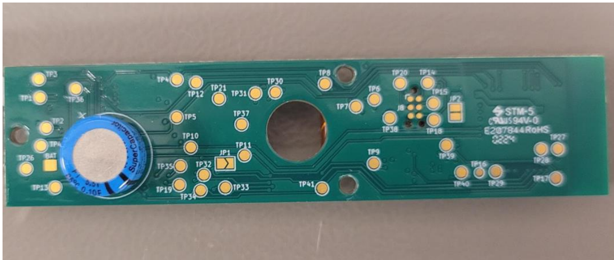
Figure 3: PCB Bottom View Photo
