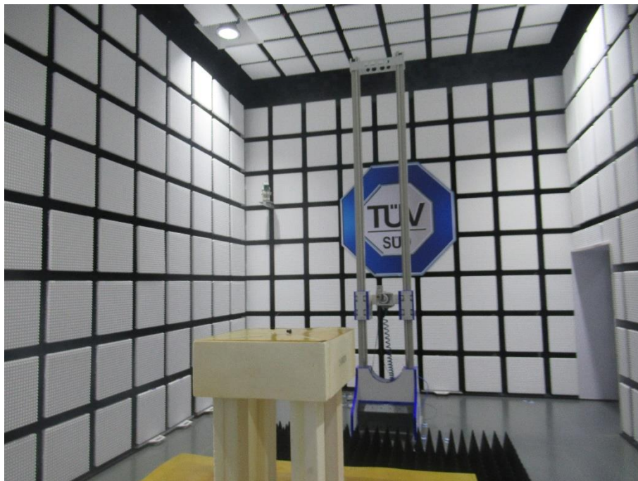
18GHz-40GHz RSE Setup
