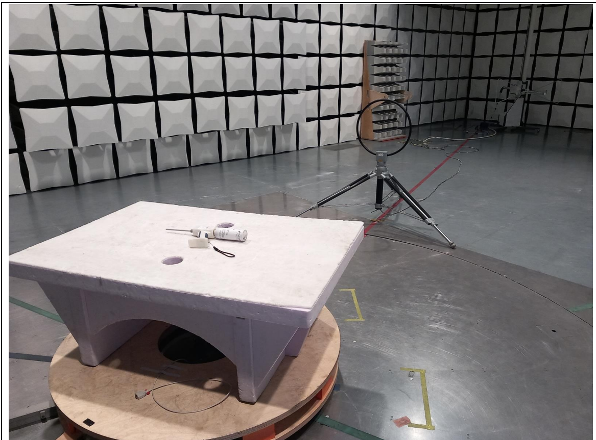
Test Setup: Radiated Measurements (9 kHz - 30 MHz) Parallel polarization
