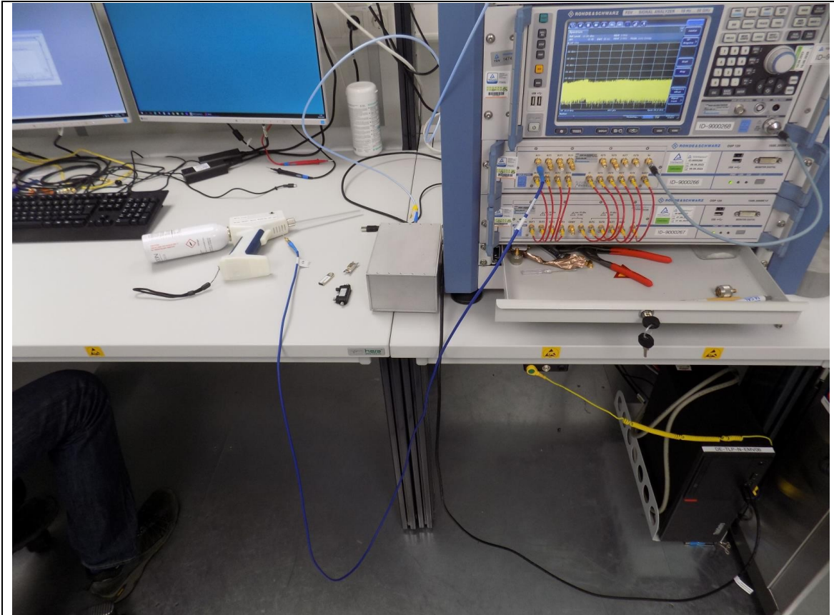
Test Setup: Conducted Measurements
