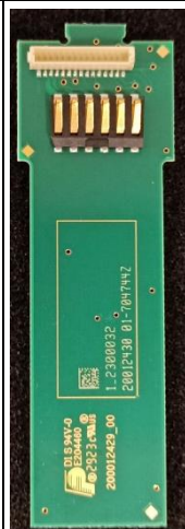
Picture 7 : Pushbutton-PCB Bottom view
