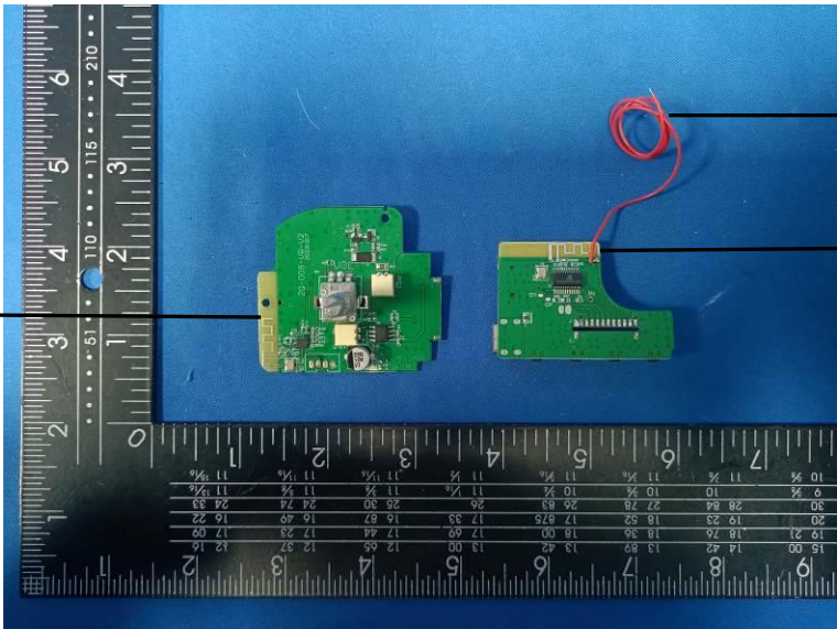
Receiving Antenna
