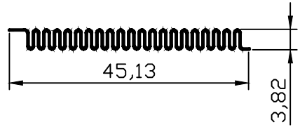
TX Antenna(Wire diameter0.5mm)
