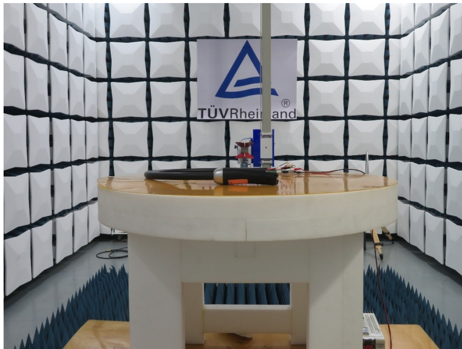
Setup of Radiated Spurious Emissions above 1GHz
