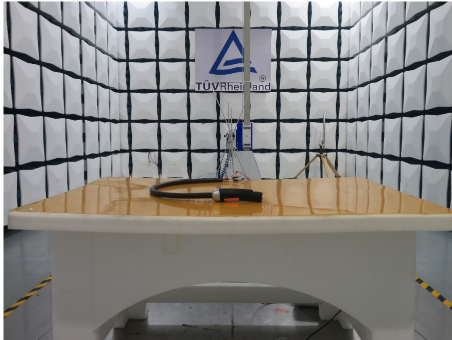
Setup of Radiated Spurious Emissions up to 1GHz
