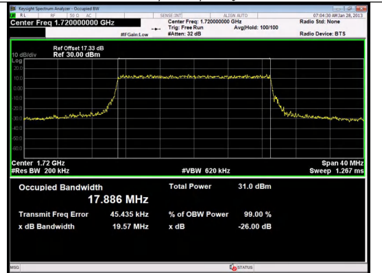
Band 4 20MHz/1720.0/Low QPSK 100@0
