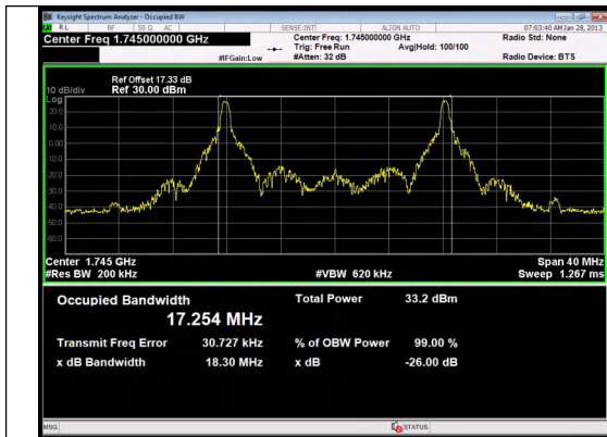
Band 4 20MHz/1745.0/High 16QAM 100@0
