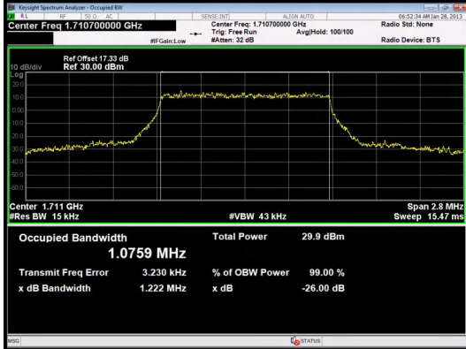
Band 4 1.4MHz/1710.7/Low 16QAM 6@0
