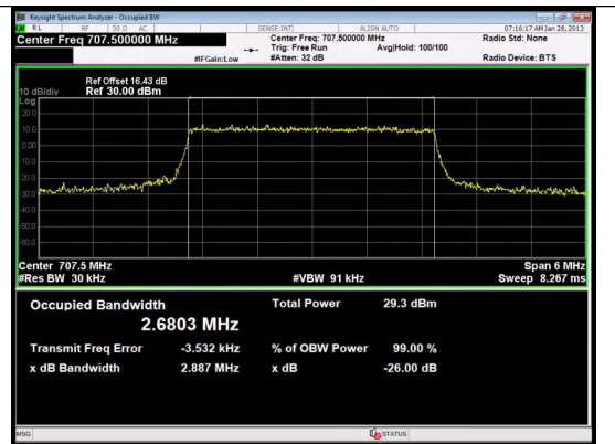
Band 12 3MHz/707.5/Mid 16QAM 15@0
