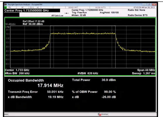
Band 4 20MHz/1732.5/Mid QPSK 100@0
