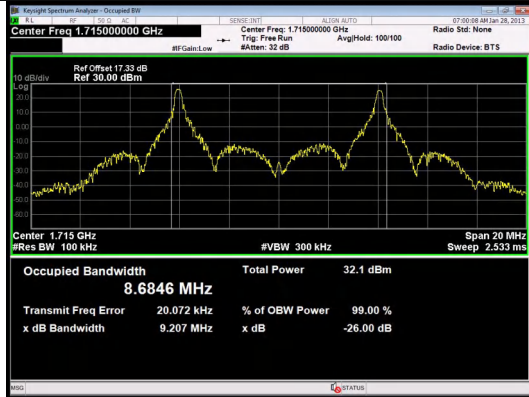
Band 4 10MHz/1715.0/Low 16QAM 50@0
