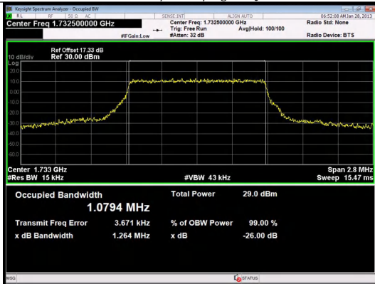
Band 4 1.4MHz/1732.5/Mid 16QAM 6@0
