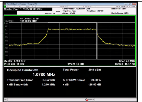
Band 4 1.4MHz/1732.5/Mid QPSK 6@0
