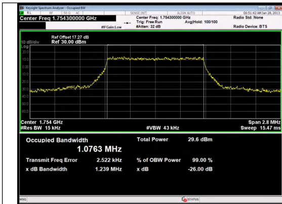
Band 4 1.4MHz/1754.3/High 16QAM 6@0
