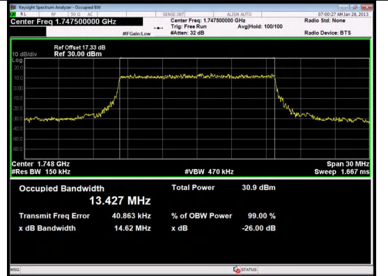
Band 4 15MHz/1747.5/High QPSK 75@0
