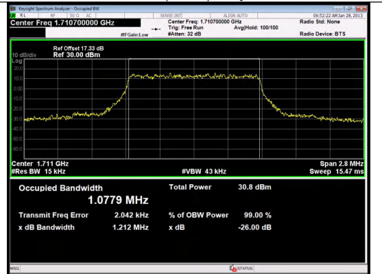
Band 4 1.4MHz/1710.7/Low QPSK 6@0
