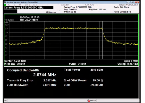
Band 4 3MHz/1753.5/High QPSK 15@0
