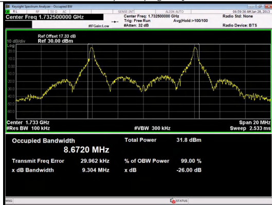
Band 4 10MHz/1732.5/Mid 16QAM 50@0
