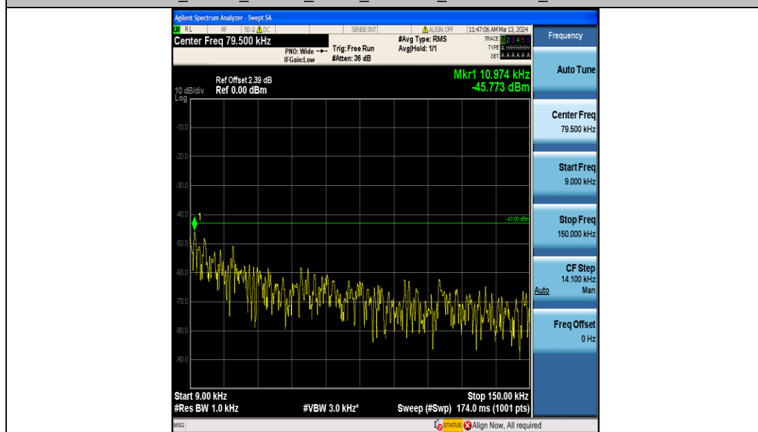
Band4_20MHz_QPSK_20300_100RB#0_0.009~0.15_0.009~0.15
