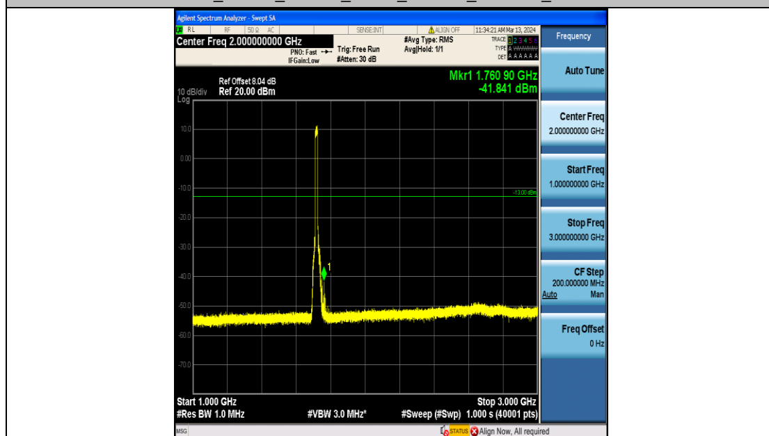
Band4_15MHz_16QAM_20025_75RB#0_1000~3000_1000~3000
