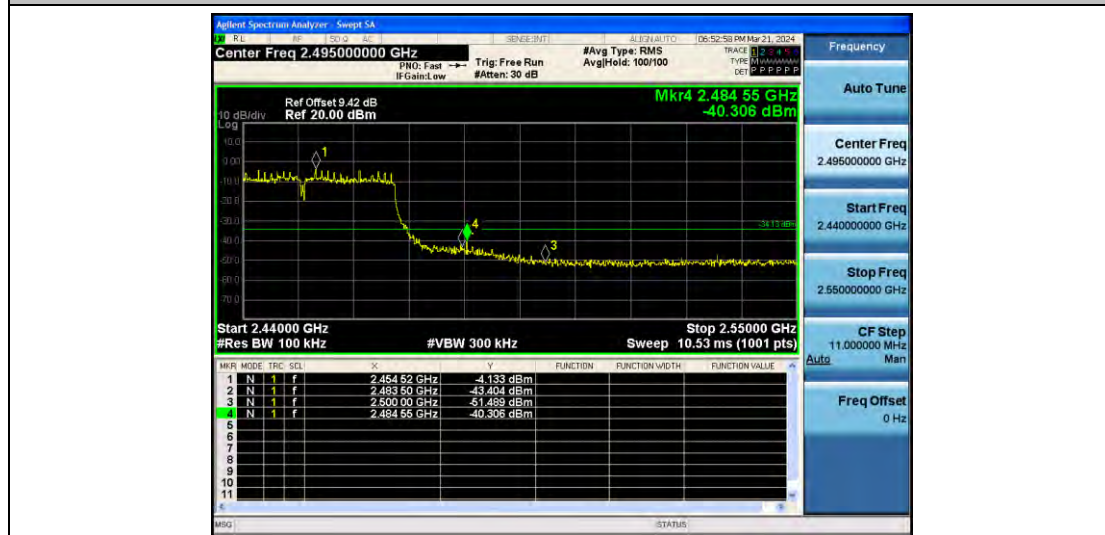
11N40MIMO_Ant1_High_2452
