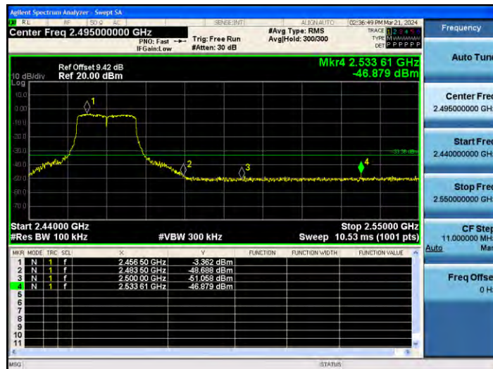
11G_Ant2_High_2462
