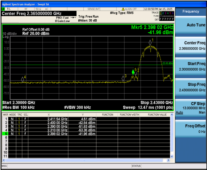
11B_Ant2_Low_2412
