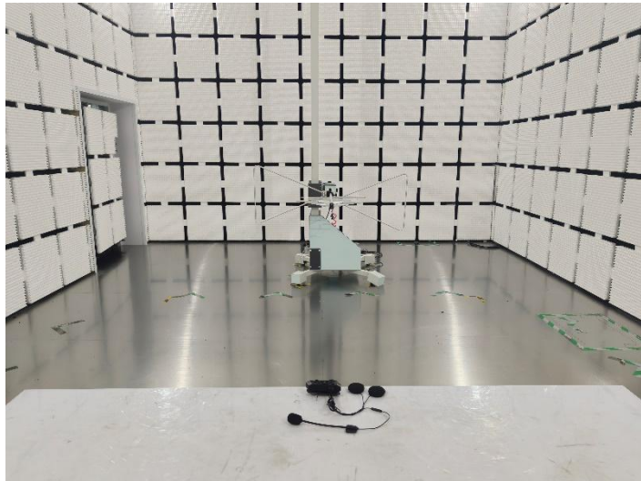
Radiated Emission
