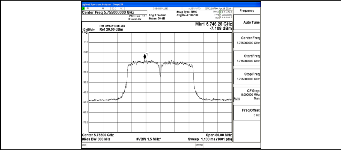
11AC40MIMO-Ant2-5755-PASS
