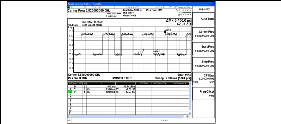
NTNV-11AC20MIMO-Ant2-5825
