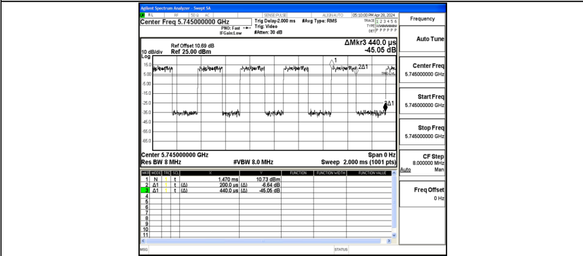
NTVN-11AC20MIMO-Ant2-5745
