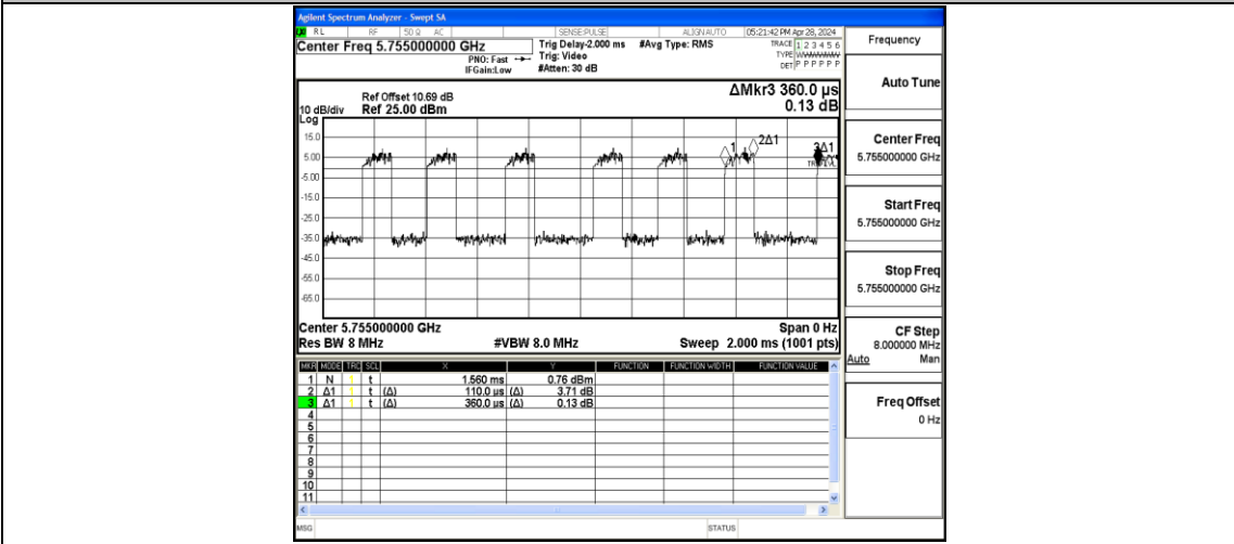
NTNV-11AC40MIMO-Ant2-5755
