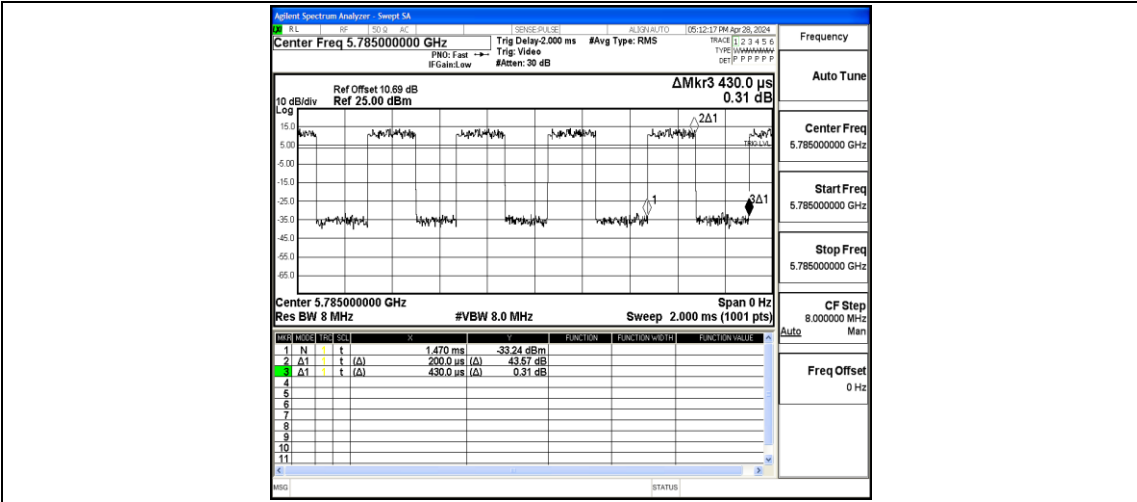
NTNV-11AC20MIMO-Ant1-5785
