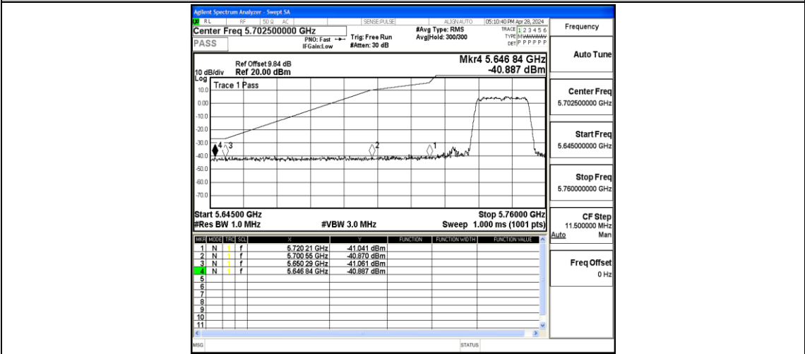
11AC20MIMO-Ant2-5745-PASS
