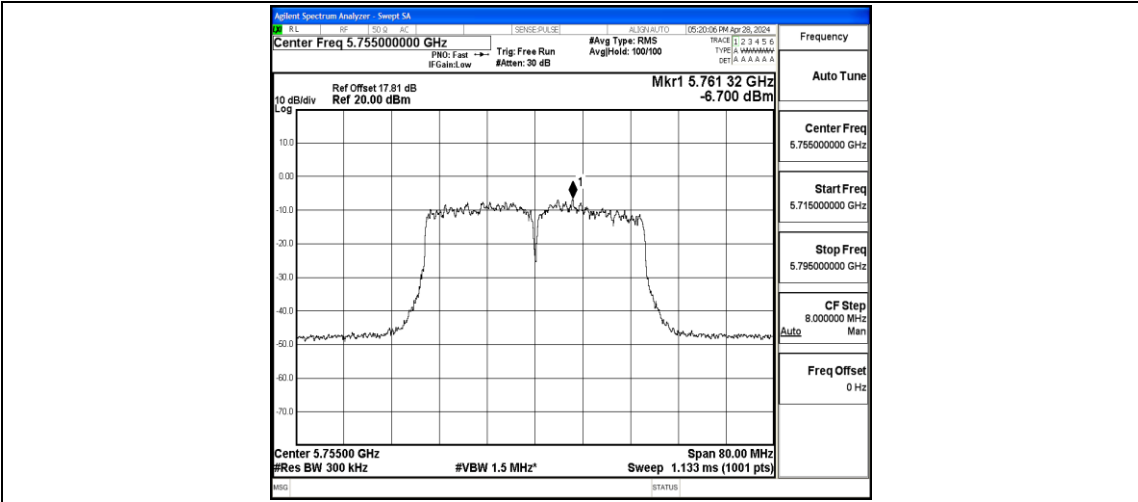
11AC40MIMO-Ant1-5755-PASS
