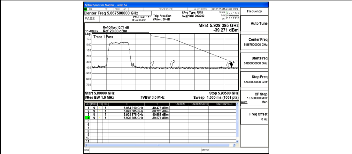
11AC20MIMO-Ant1-5825-PASS
