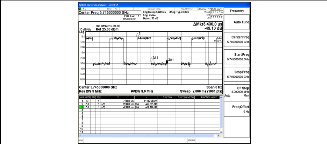
NTVN-11AC20MIMO-Ant1-5745
