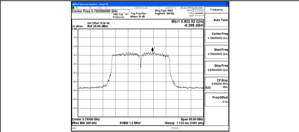
11AC40MIMO-total-5795-PASS
