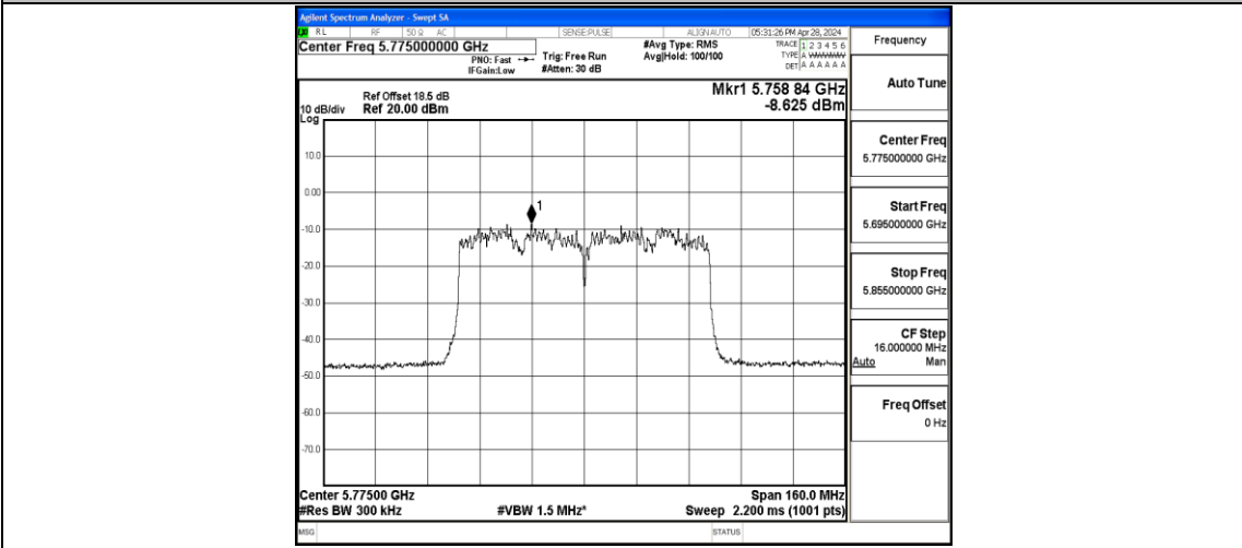
11AC80MIMO-total-5775-PASS
