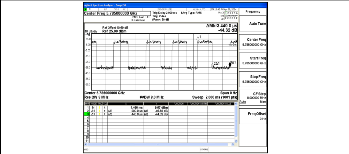
NTNV-11AC20MIMO-Ant2-5785
