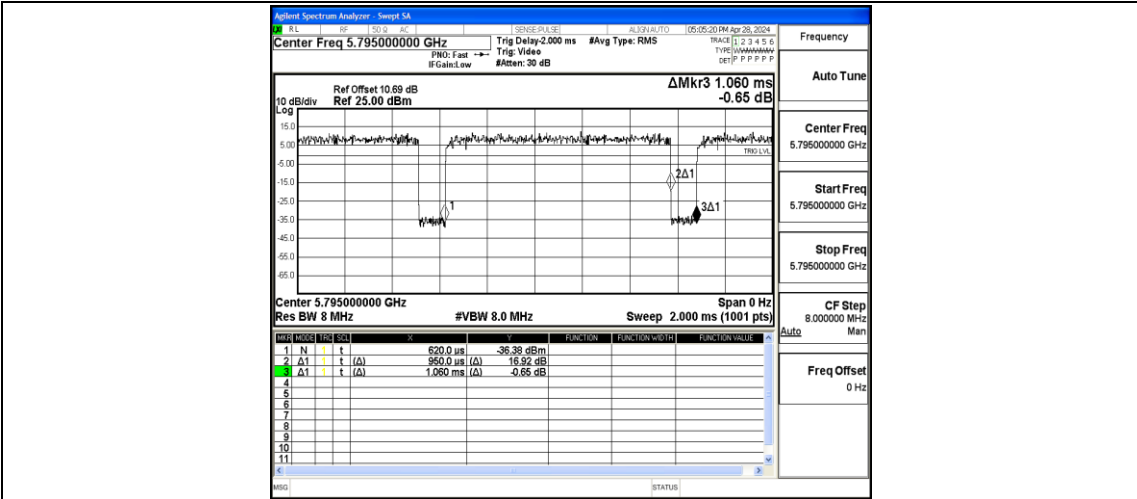
NTVN-11N40MIMO-Ant2-5795
