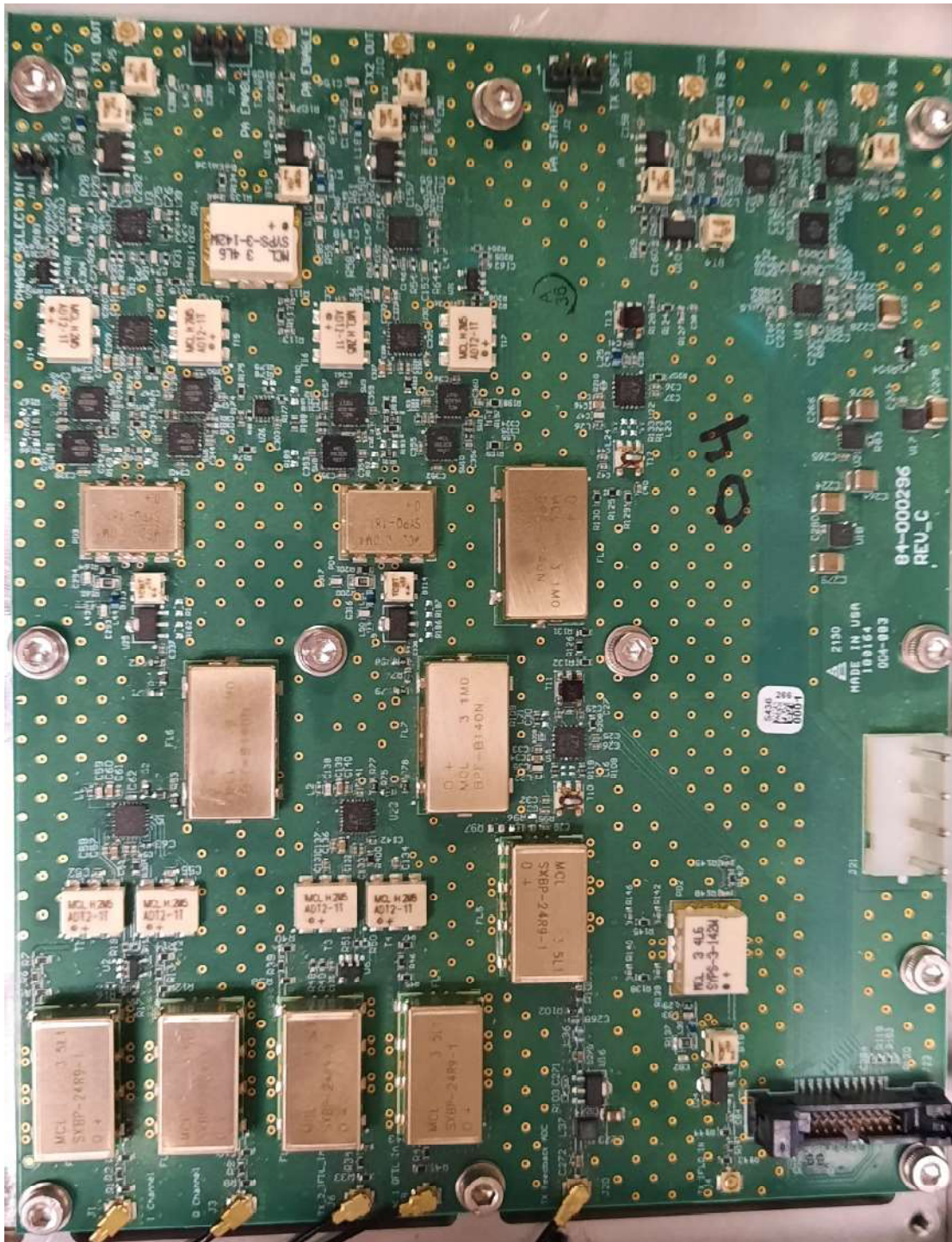
Transmit Board – Top
