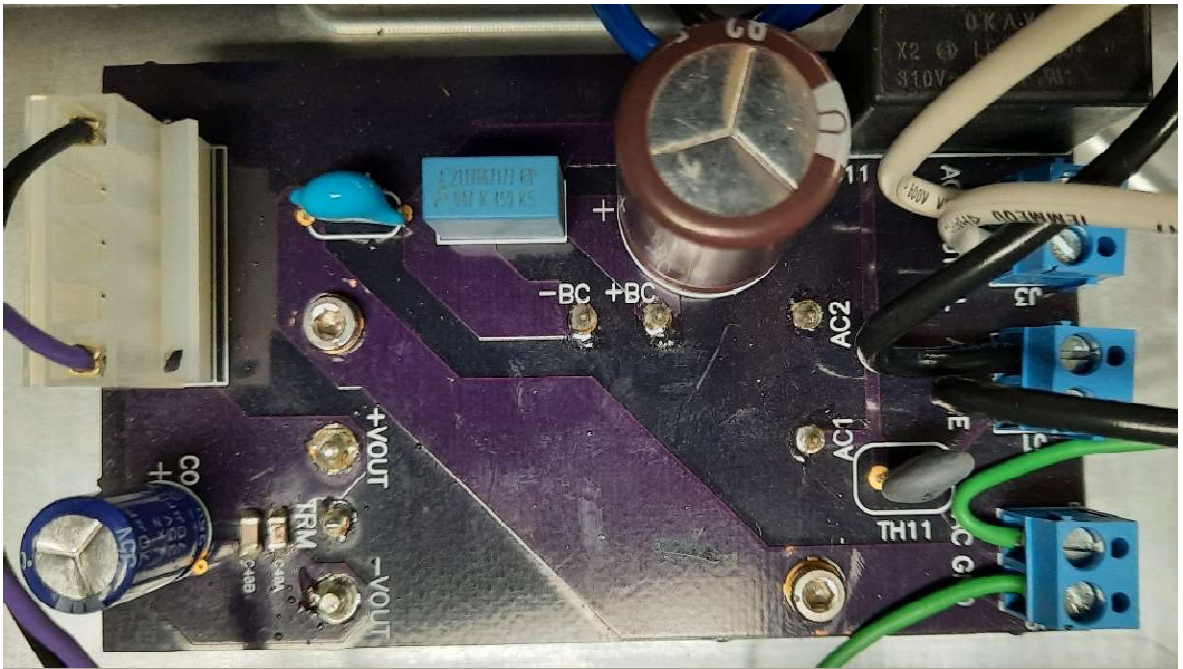
12V Power Supply – Top
