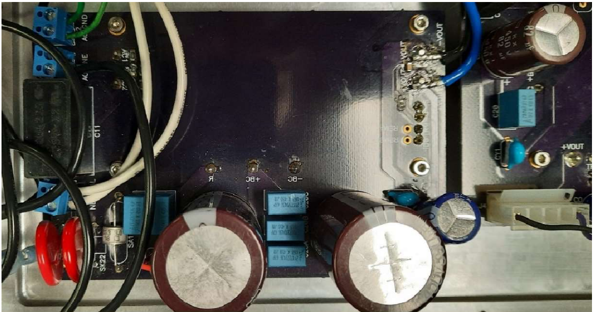
48V Power Supply – Top
