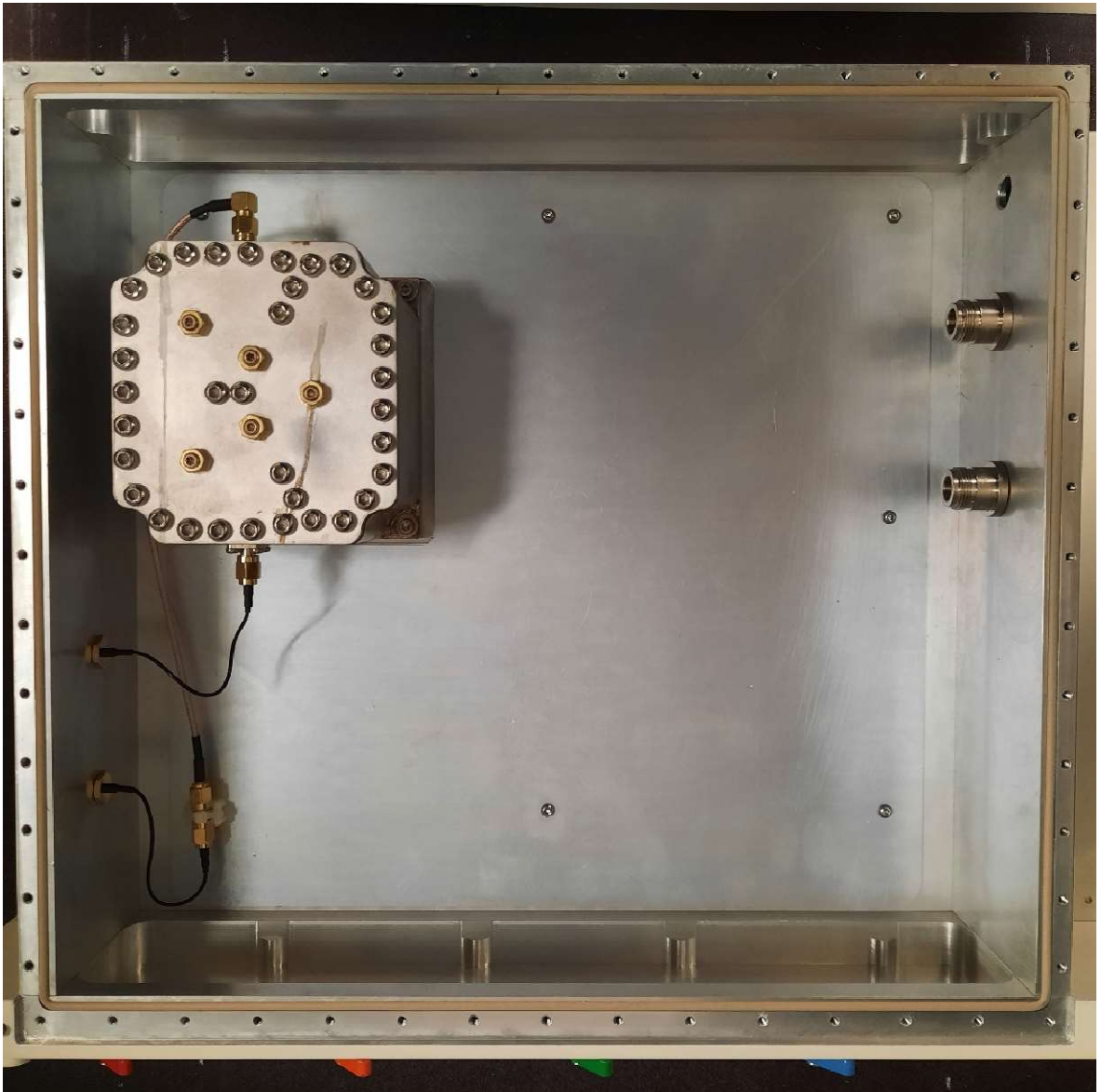
Duplexer Module Bottom Cover Removed
