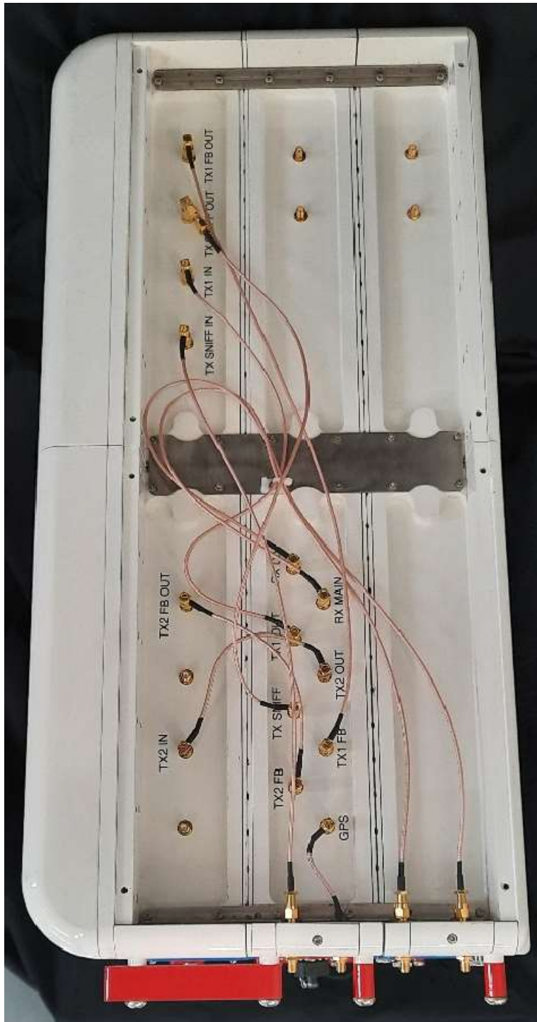
Right Side – Cover Removed
