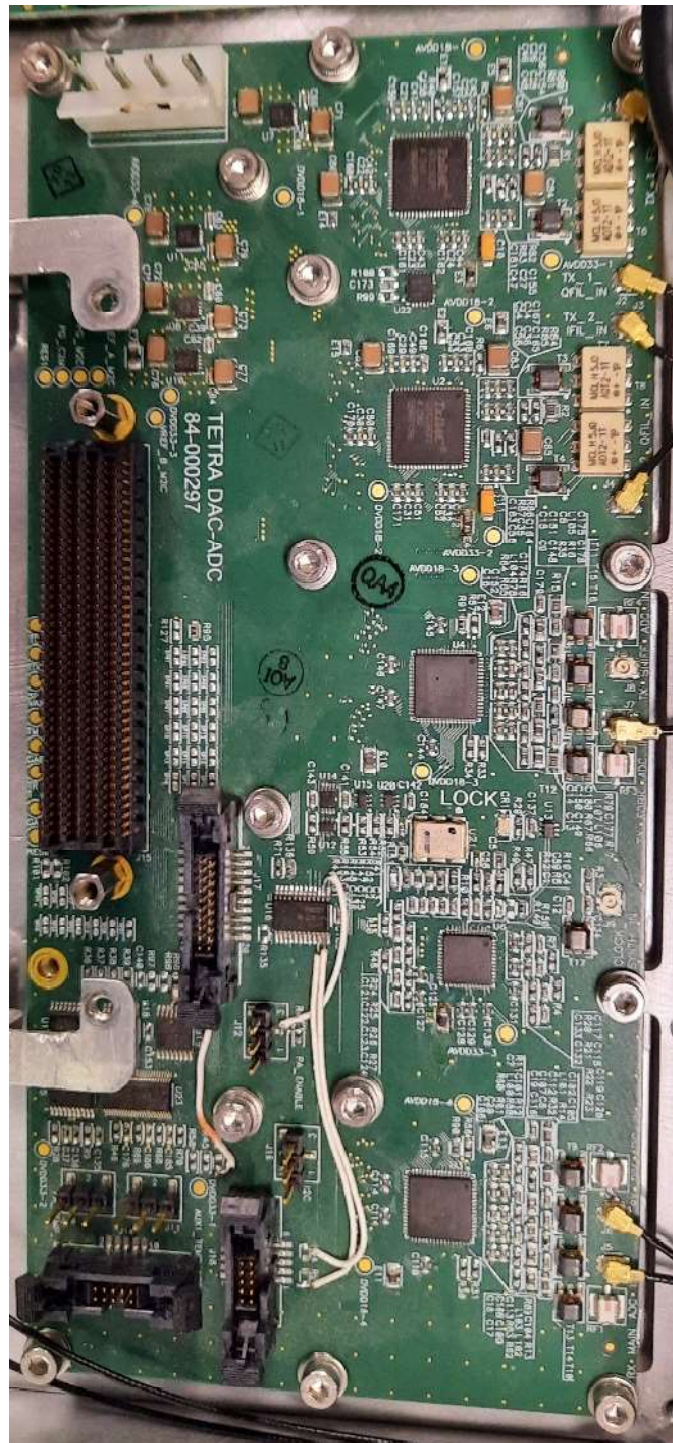
DAC_ADC Board - Top
