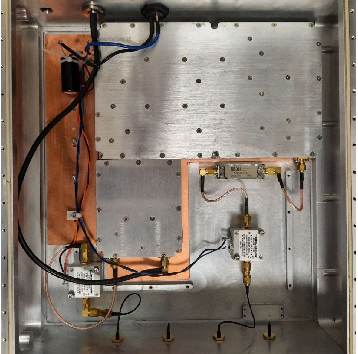
PA Module Mirror Bottom Cover Removed
