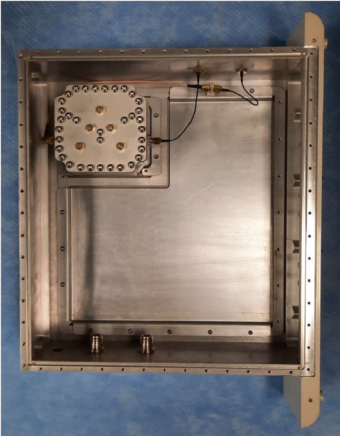
Duplexer Module Mirror Top – Cover Removed
