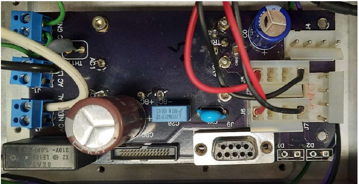
5.5V Power Supply – Top
