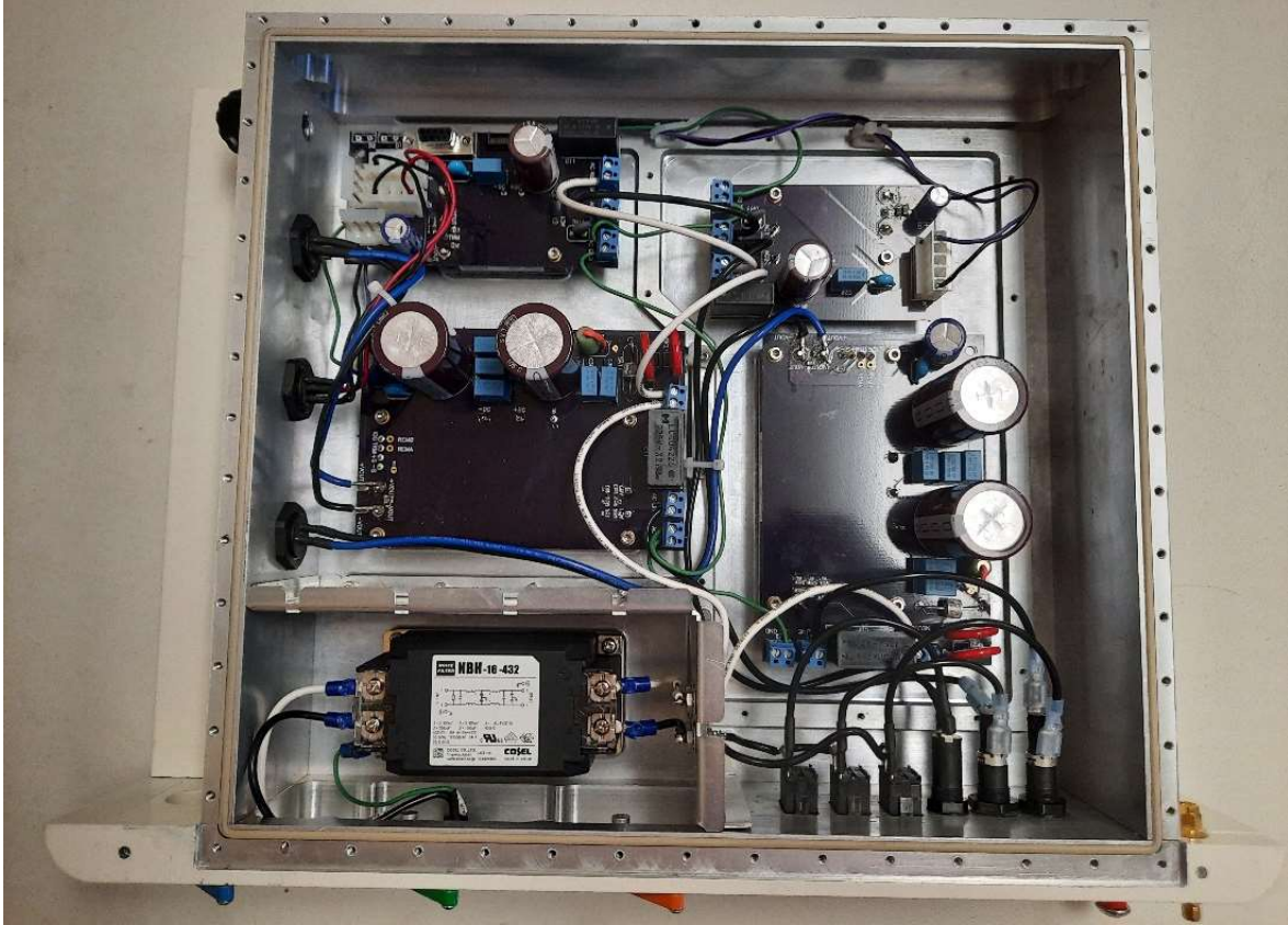
Power Module Top Cover Removed
