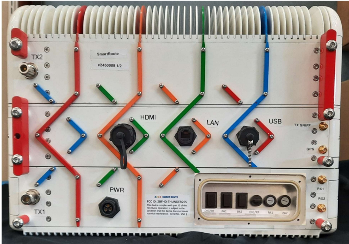
Bottom – Maintenance Panel Removed
