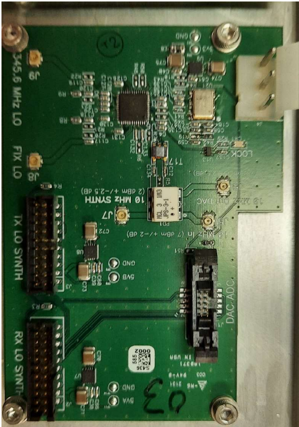
Reference Board – Top
