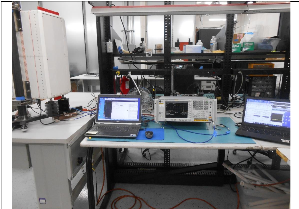
RF Conducted #2
