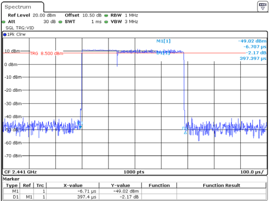
3DH1_Hopping 0.397ms
