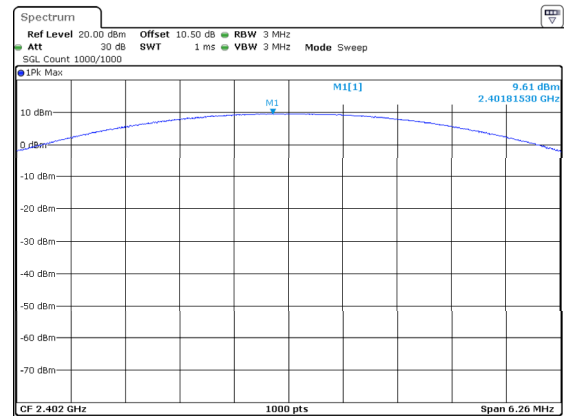
2DH1_Low 9.61dBm
