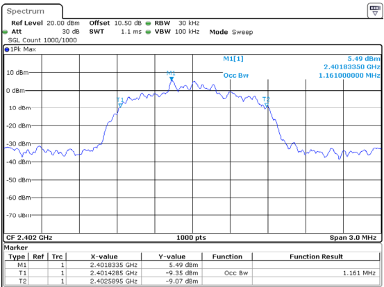
3DH1_Low 1.161MHz
