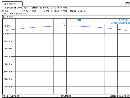
DH1_Low 9.97dBm
