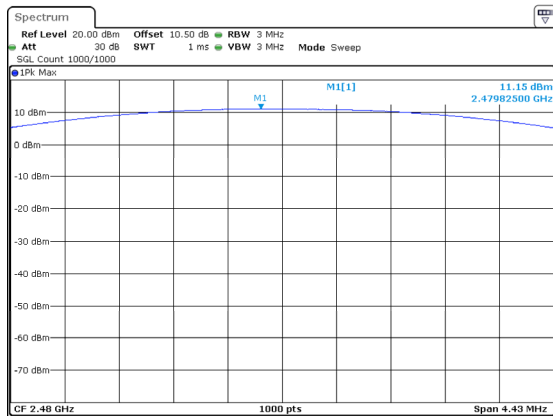
DH1_High 11.15dBm
