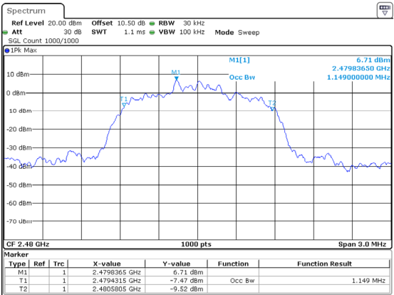
3DH1_High 1.149MHz
