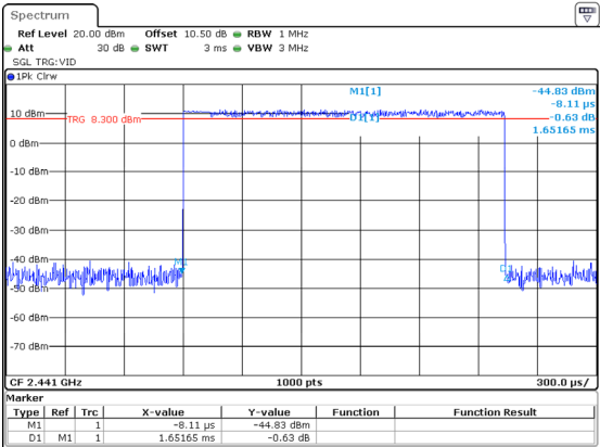
3DH3_Hopping 1.652ms
