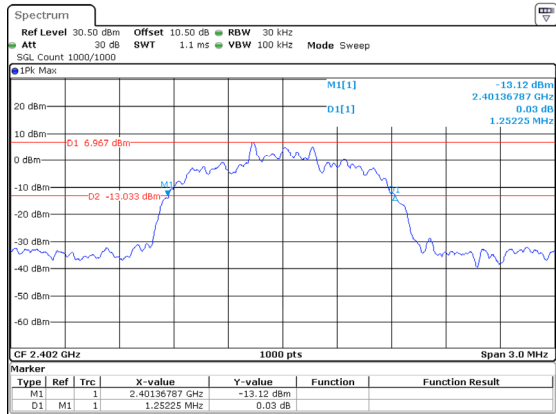
2DH1_Low 1.252MHz
