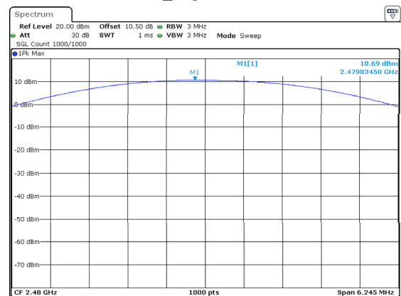
2DH1_High 10.69dBm
