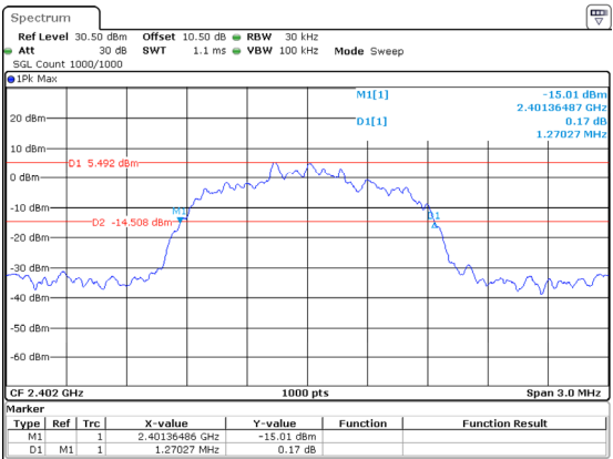
3DH1_Low 1.270MHz
