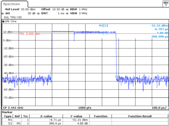
2DH1_Hopping 0.396ms
