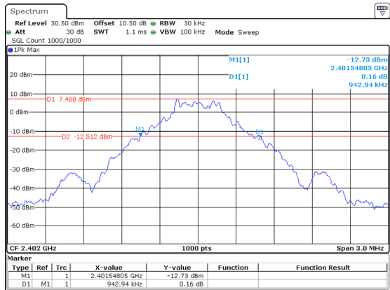
DH1_Low 0.943MHz
