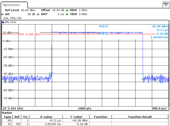
2DH3_Hopping 1.652ms
