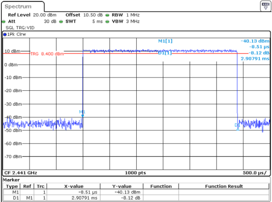
3DH5_Hopping 2.908ms
