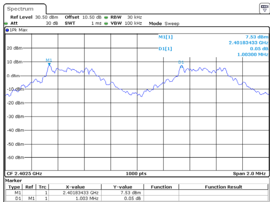
DH1_Low 1.003MHz
