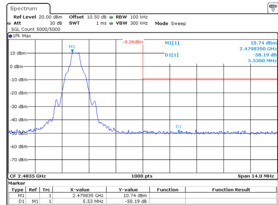
DH1_High
