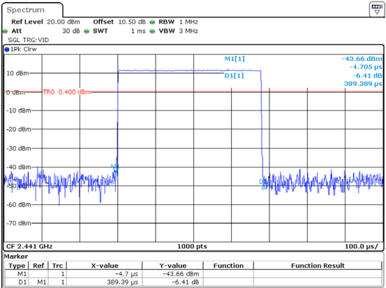
DH1_Hopping 0.389ms
