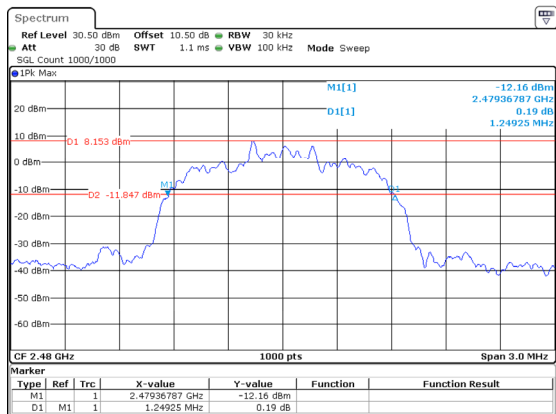
2DH1_High 1.249MHz
