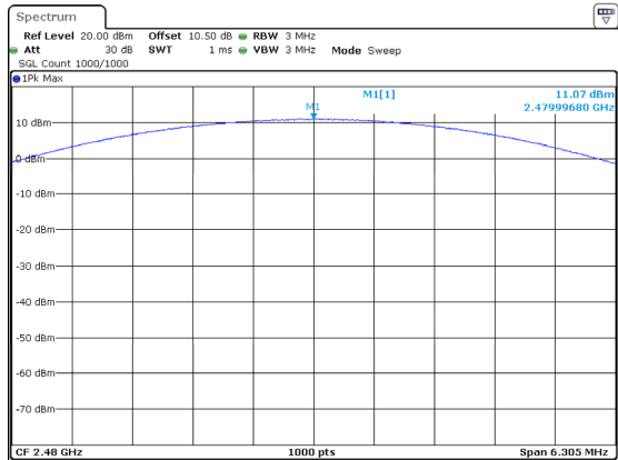
3DH1_High 11.07dBm
