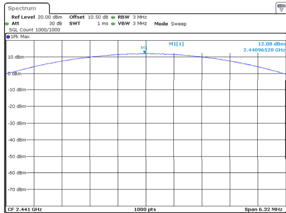
3DH1_Middle 12.08dBm
