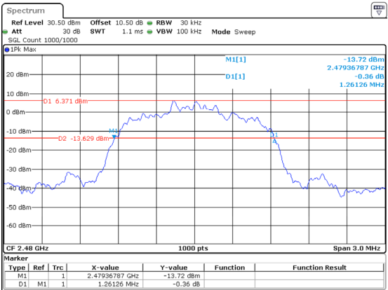
3DH1_High 1.261MHz
