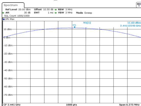
2DH1_Middle 11.63dBm
