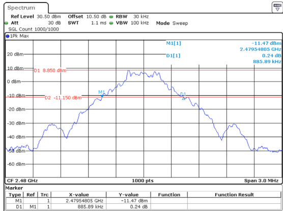
DH1_High 0.886MHz
