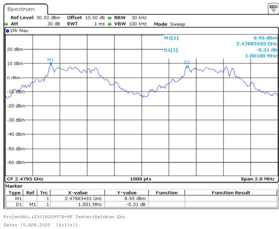
DH1_High 1.001MHz
