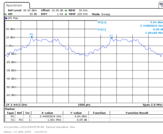
DH1_Middle 1.001MHz
