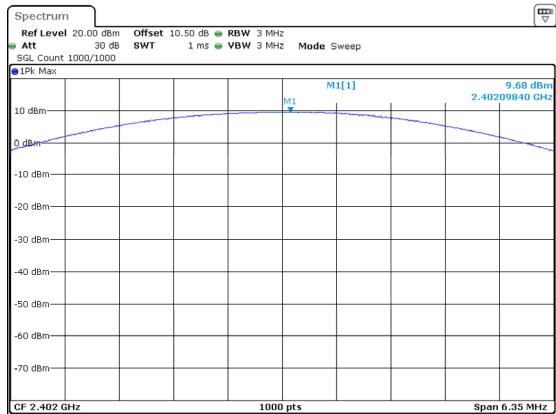
3DH1_Low 9.68dBm
