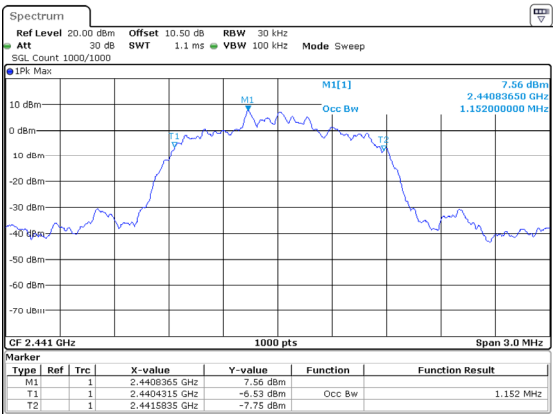
3DH1_Middle 1.152MHz
