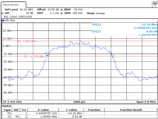
3DH1_Middle 1.264MHz
