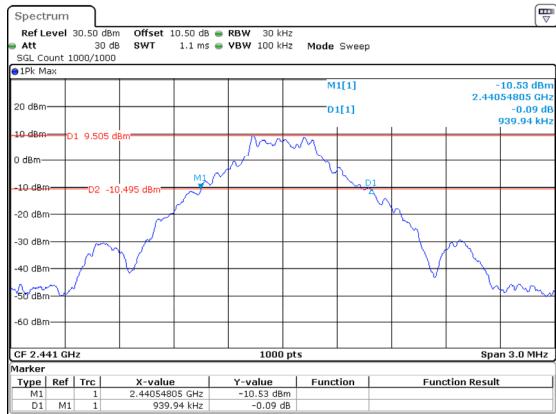
DH1_Middle 0.940MHz
