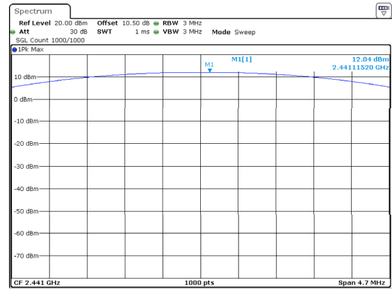
DH1_Middle 12.04dBm
