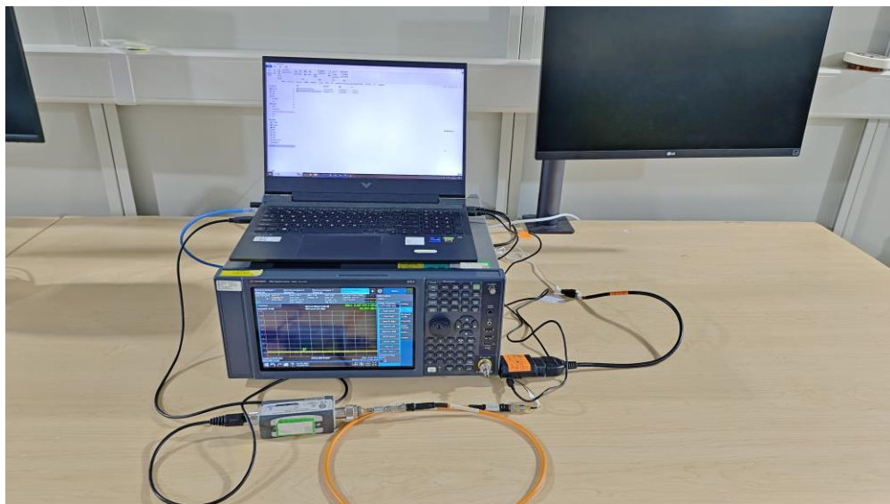
Description: Conducted Test Setup for Wi-Fi
