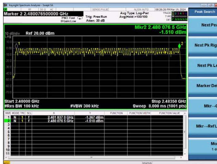
8-DPSK Modulation
