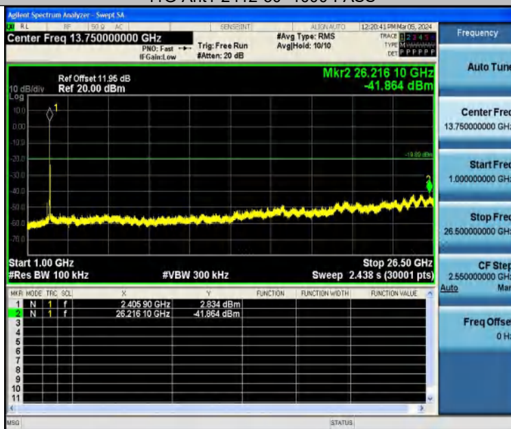
11G-Ant1-2412-1000~26500-PASS
