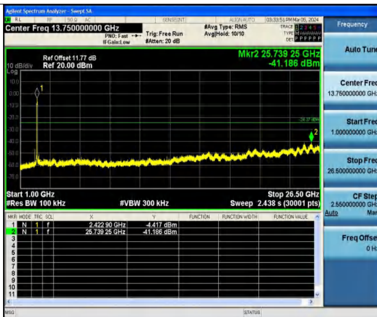
11N40SISO-Ant1-2437-1000~26500-PASS
