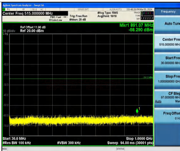
11N40SISO-Ant1-2452-30~1000-PASS
