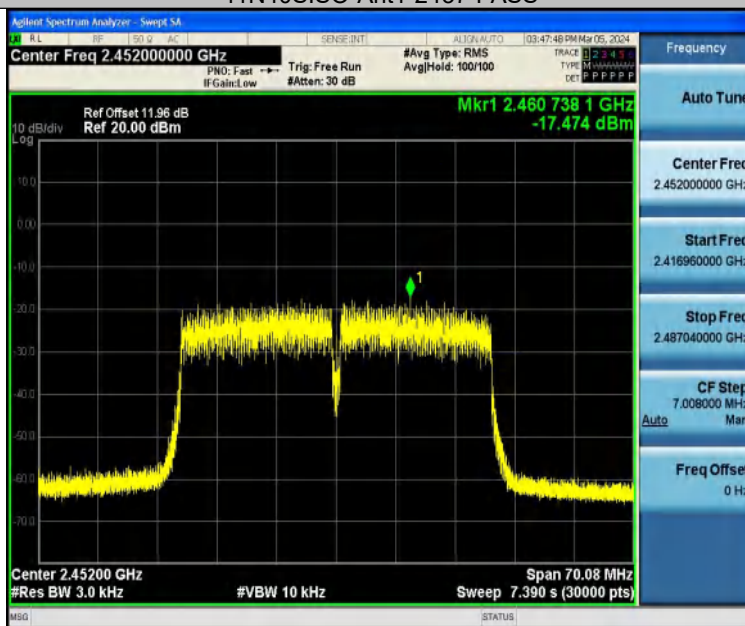
11N40SISO-Ant1-2452-PASS
