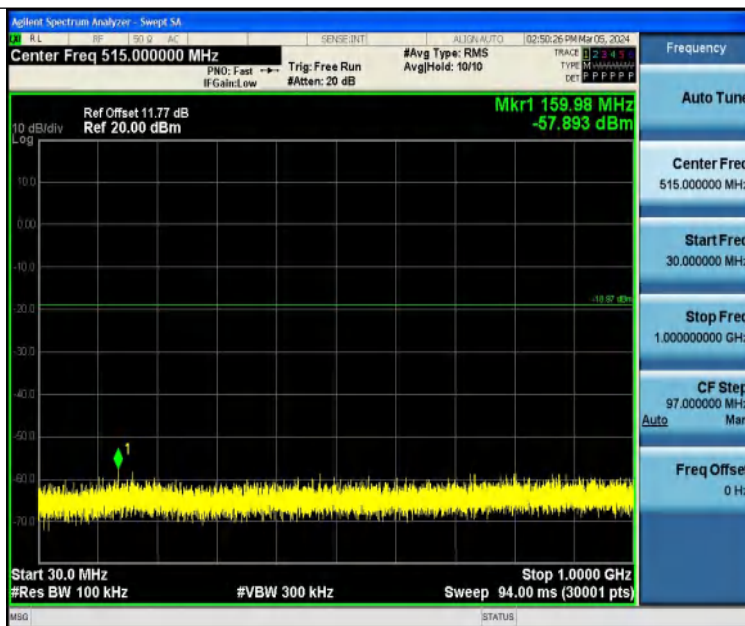
11N20SISO-Ant1-2437-30~1000-PASS
