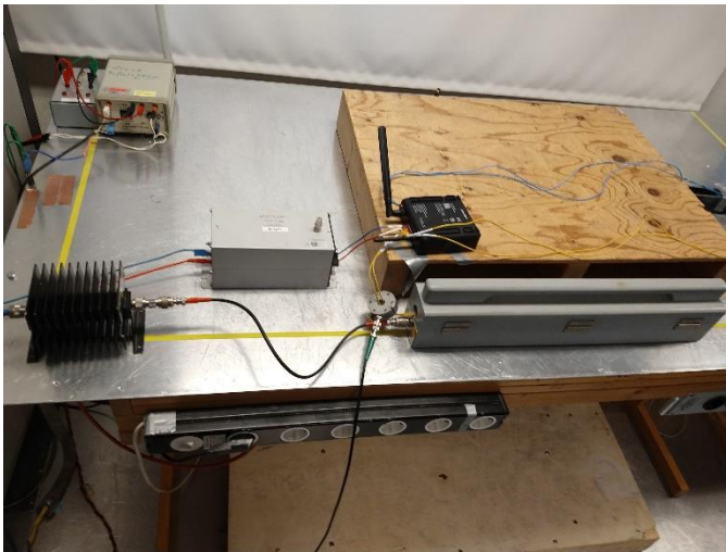
Conducted RF Disturbance Immunity (Relay NO)
