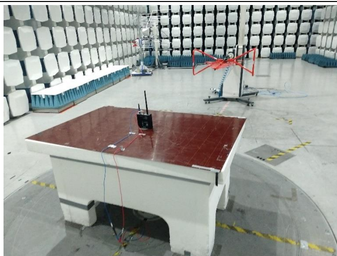
Radiated Emissions (Below 1GHz) (FCC CFR 47 Subpart 15B)
