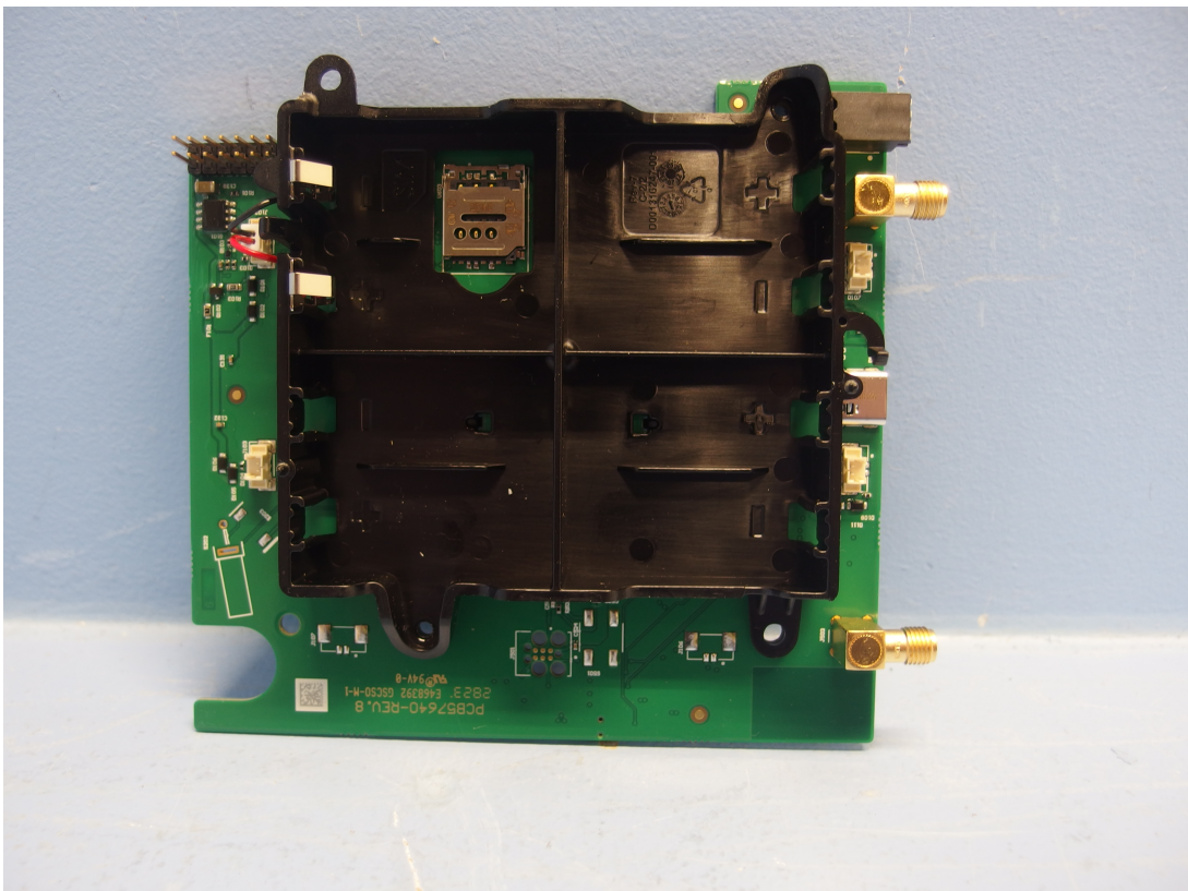
Enclosure removed
