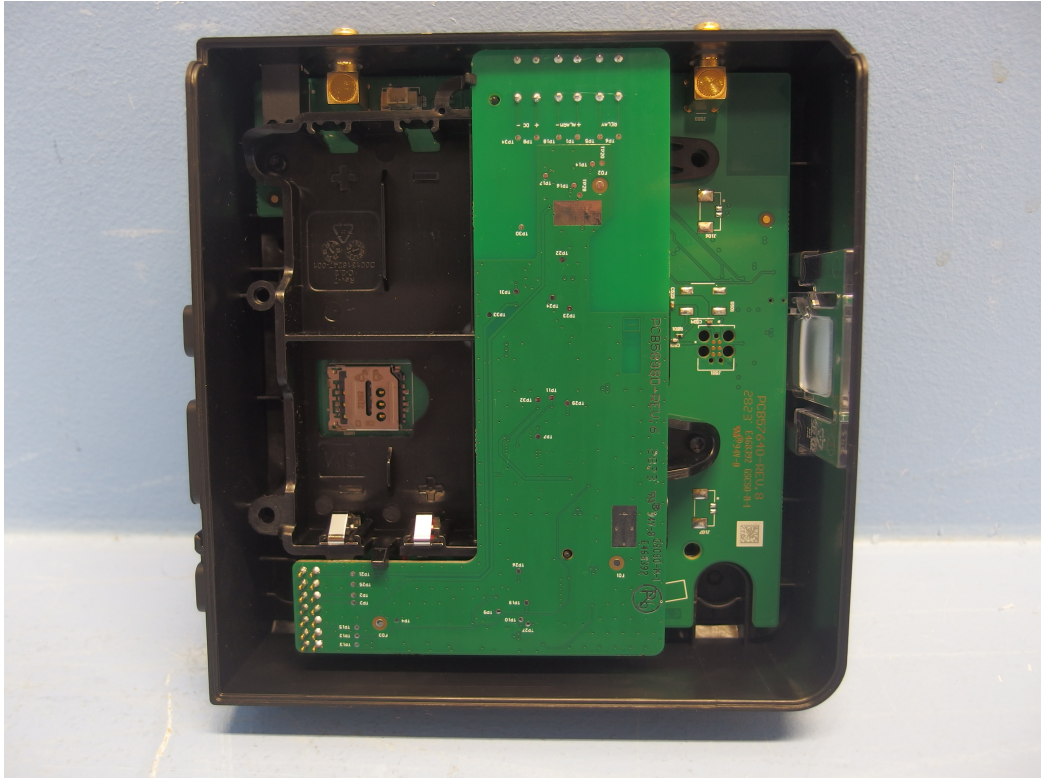
Front cover removed, extra PCB for DC mains visible
