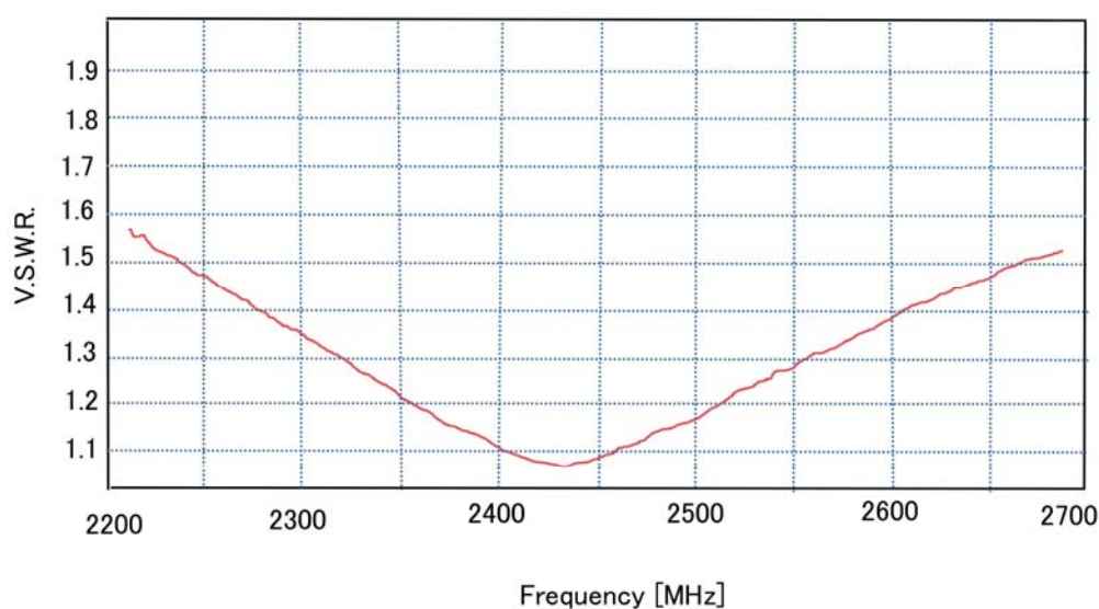
Fig.1 驻波比 VSWR
