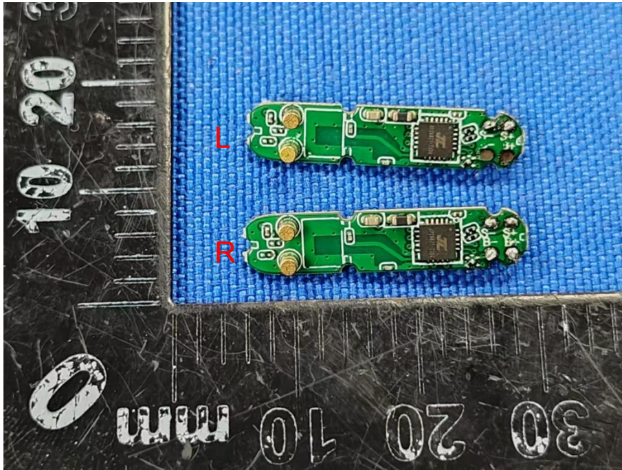
Figure 3. PCB view of headphone
