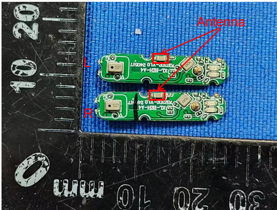
Figure 4. PCB view of headphone
