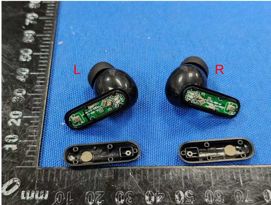
Figure 1. Internal view of headphone
