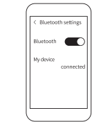
connection succeeded
