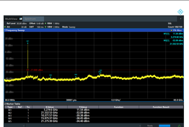
11ac (HT20) CH56
