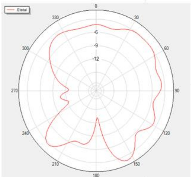
Phi=0 Freq=2400MHz
