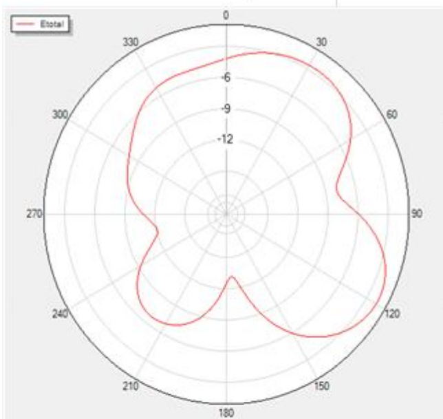
Phi=0 Freq=2400MHz
