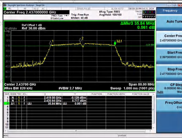
11N40SISO-Ant1-2437-PASS
