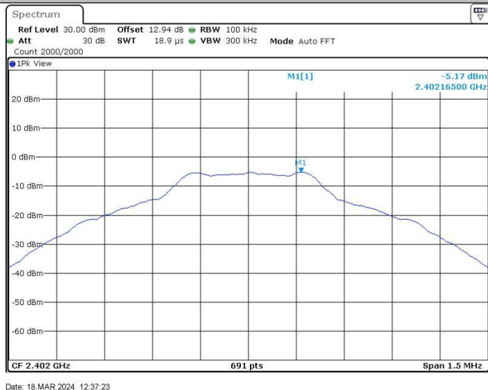
DH5_Ant1_2402_0~Reference
